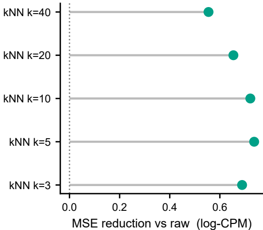
Gain over no-denoising
