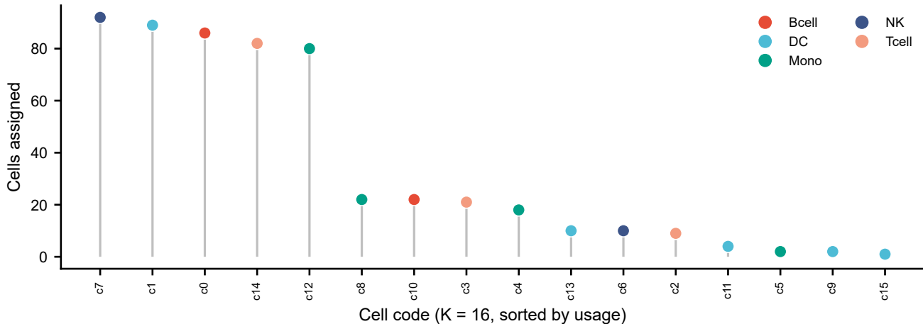
Codebook usage, coloured by dominant cell type
