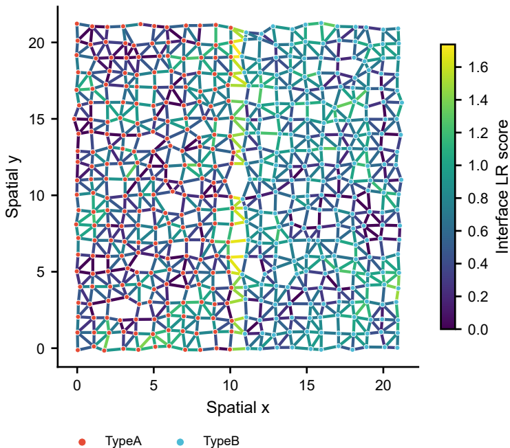
Interface graph, score of LIG_IF1_REC_IF1
