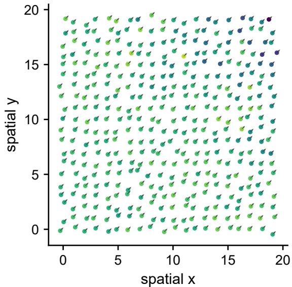
scVelo (non-spatial)
