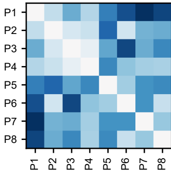
B1 mean-field Ising
