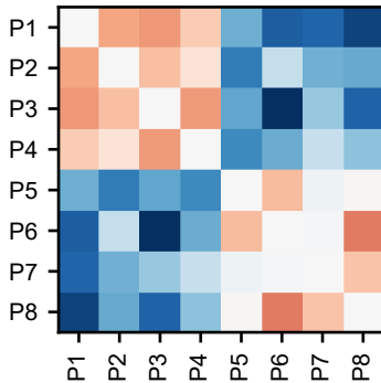
B0 pooled correlation
