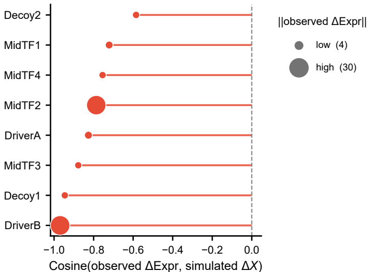
Transition S2-&gt;S3
