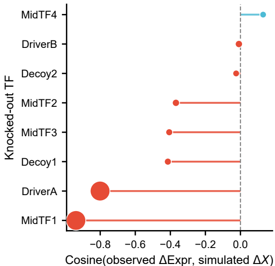
Transition S1-&gt;S2
