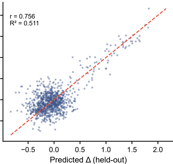
Cell-type-specific \Delta
