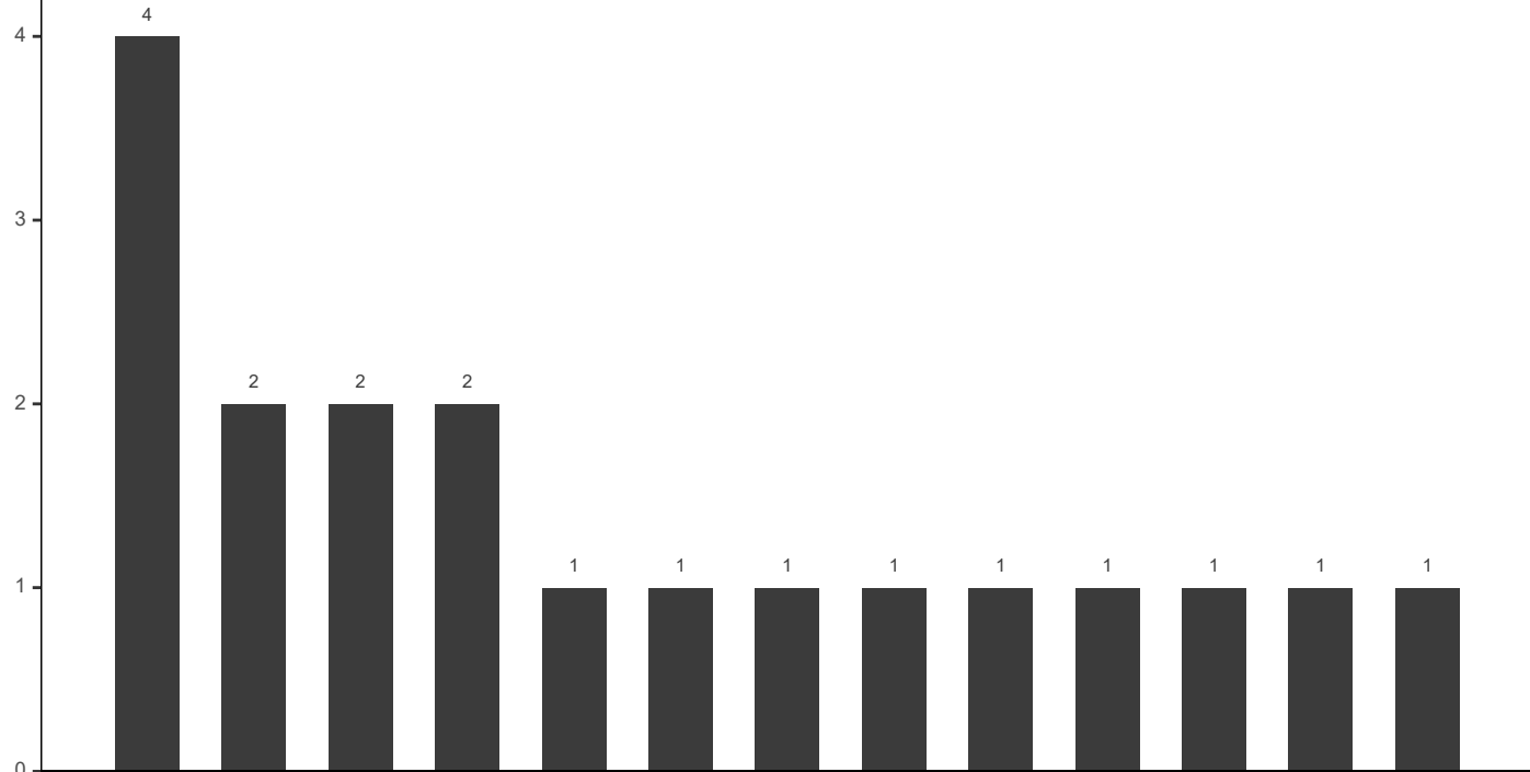
Shared features
