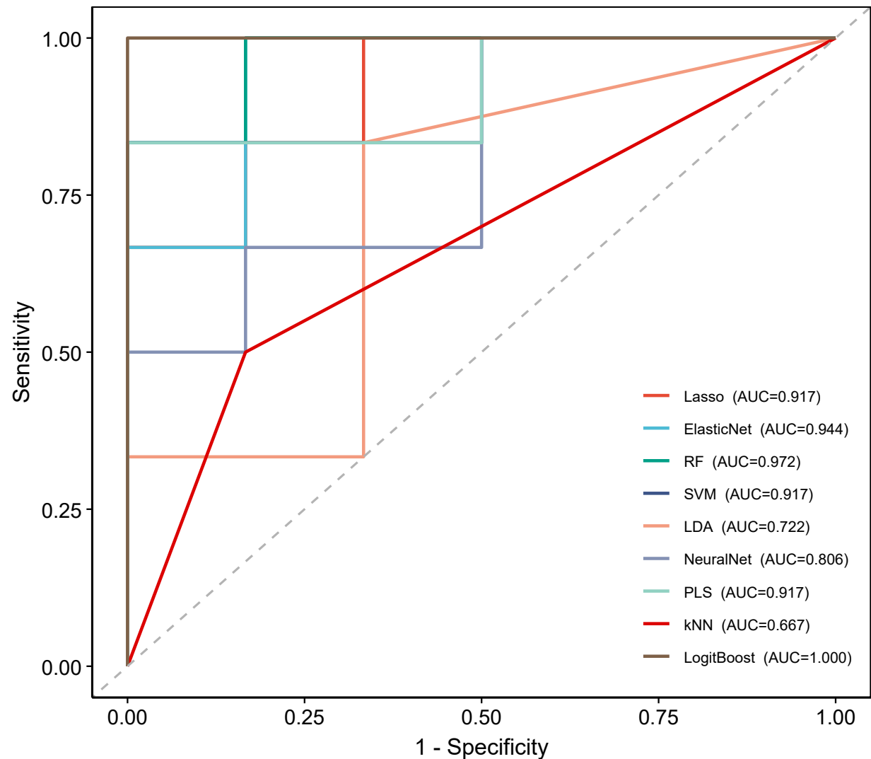
Model comparison — ROC
