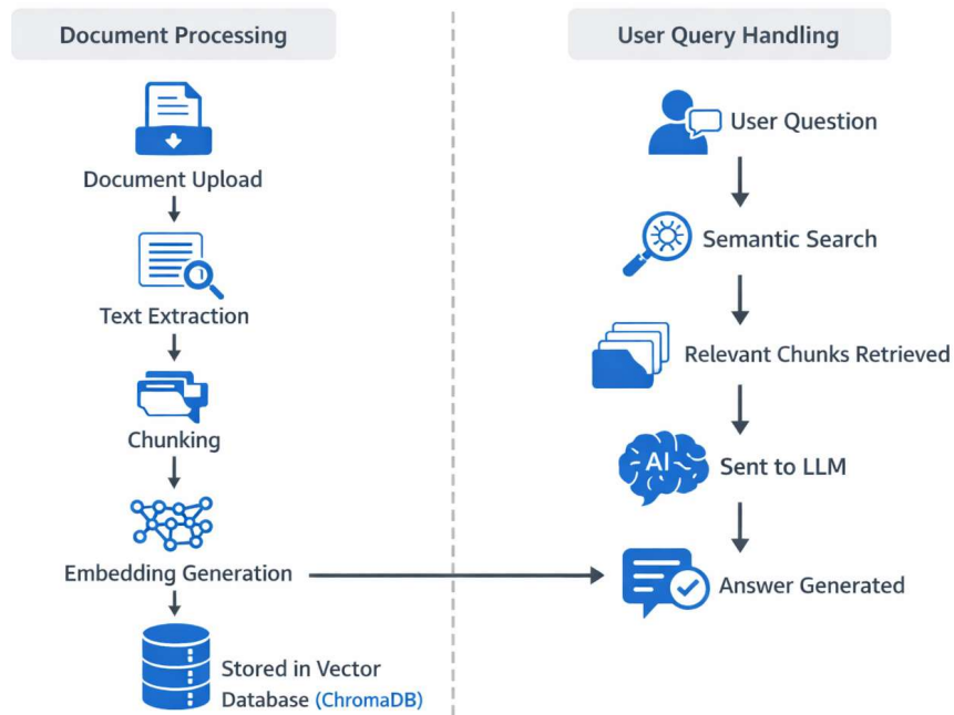
Figure 6: Left — Document processing pipeline (upload to vector database). Right — Query handling (user question to AI answer).
