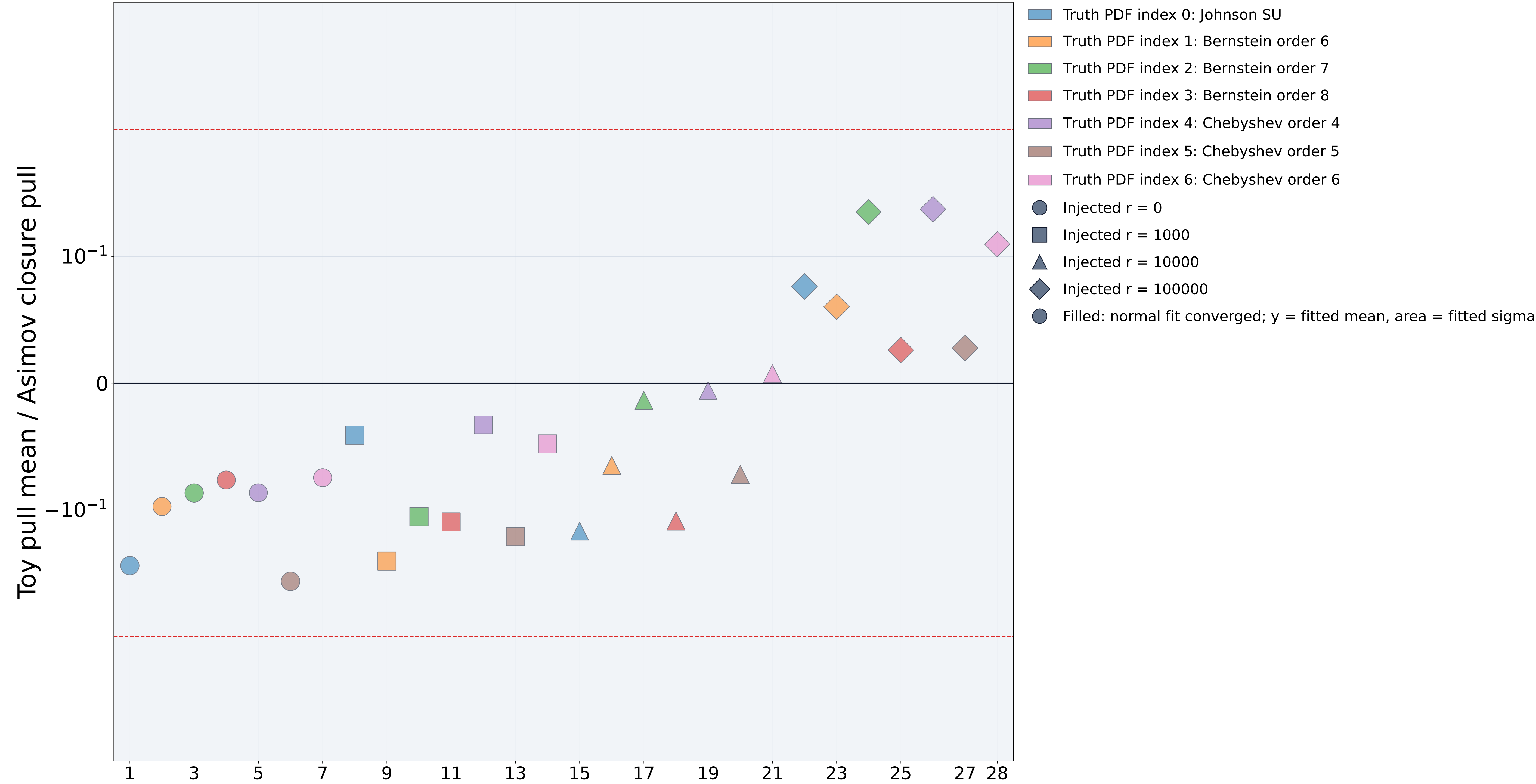
H \rightarrow Y(nS)\gamma combined
