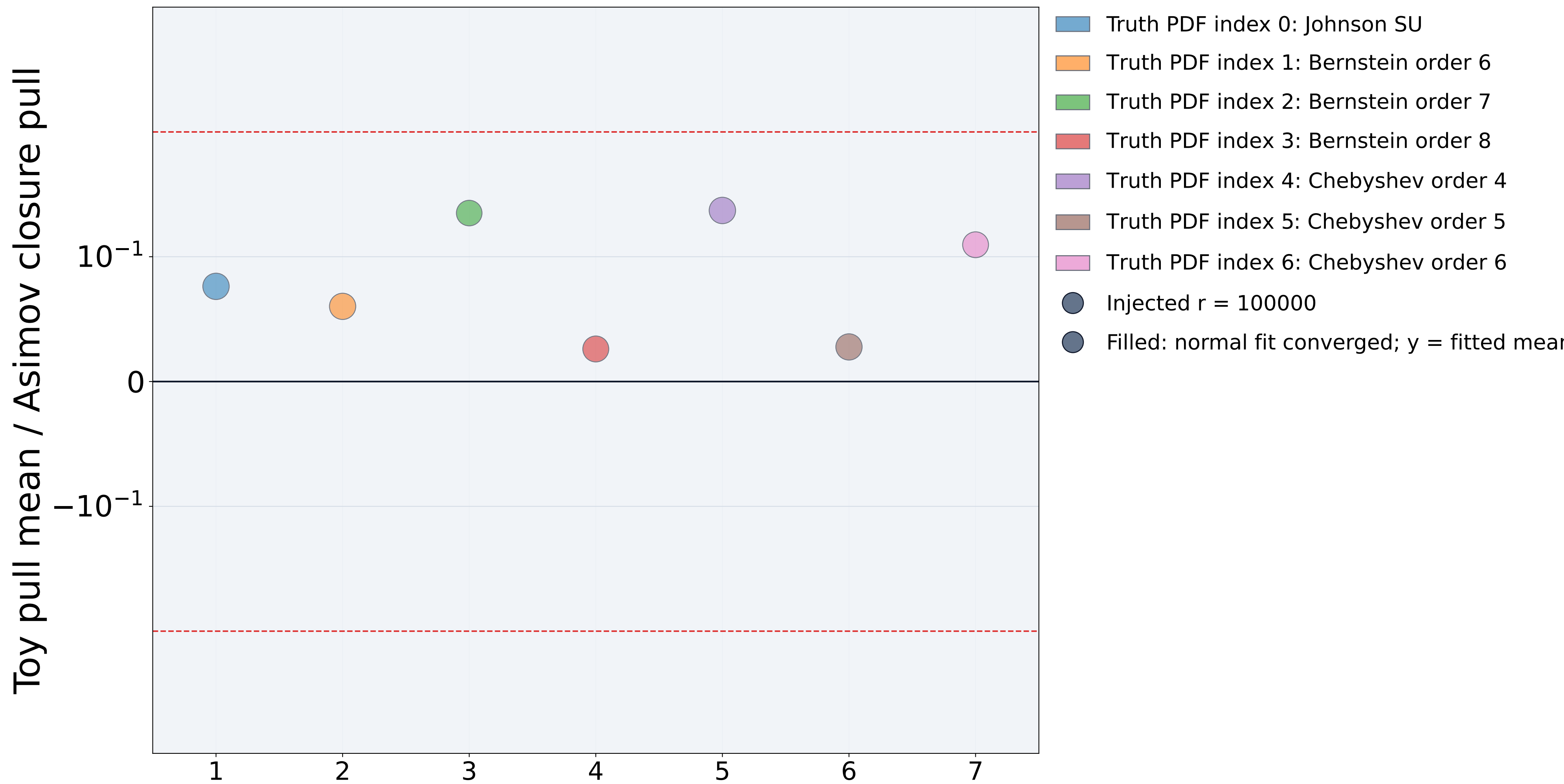
H \rightarrow Y(nS)\gamma combined
