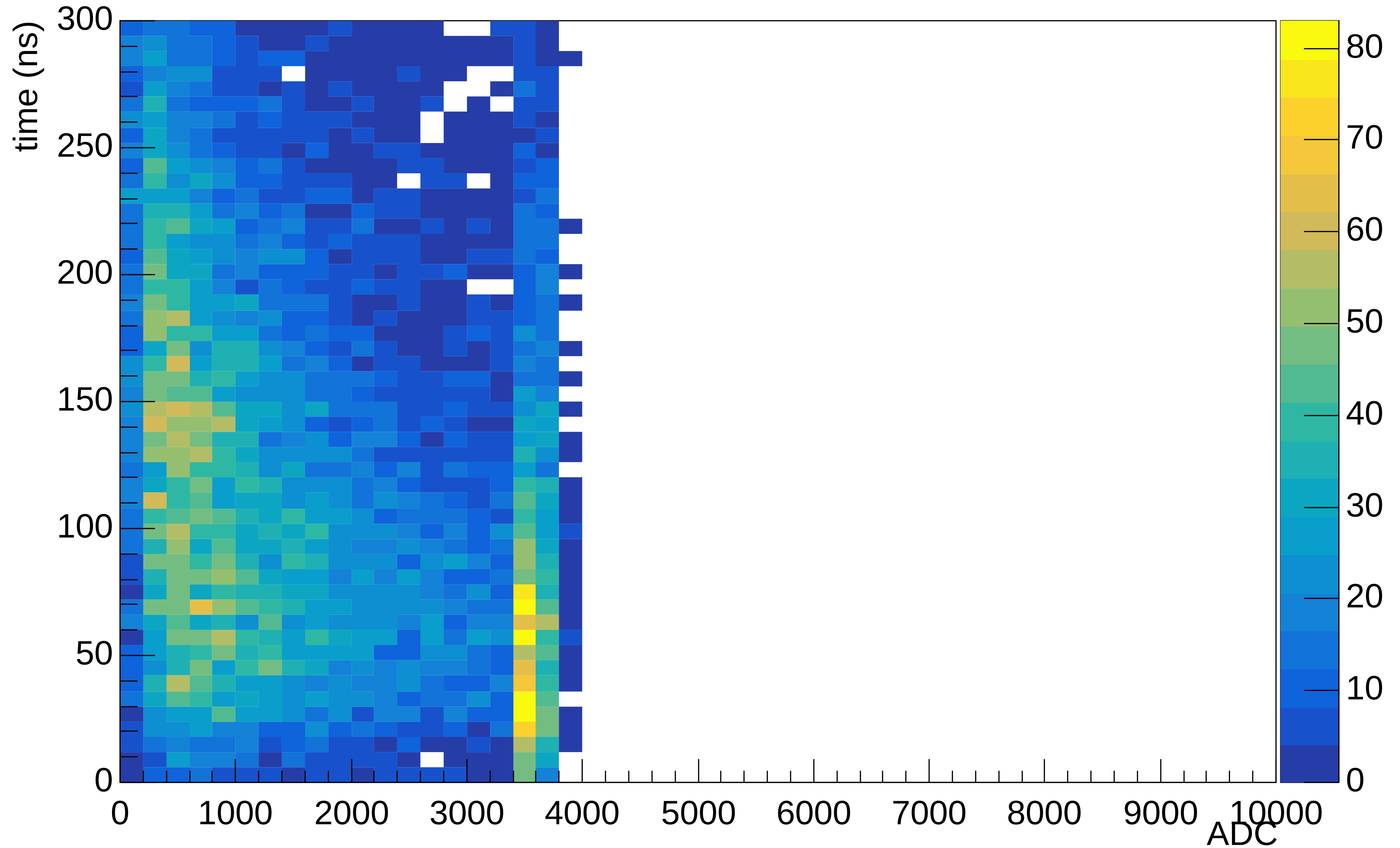
time vs ADC
