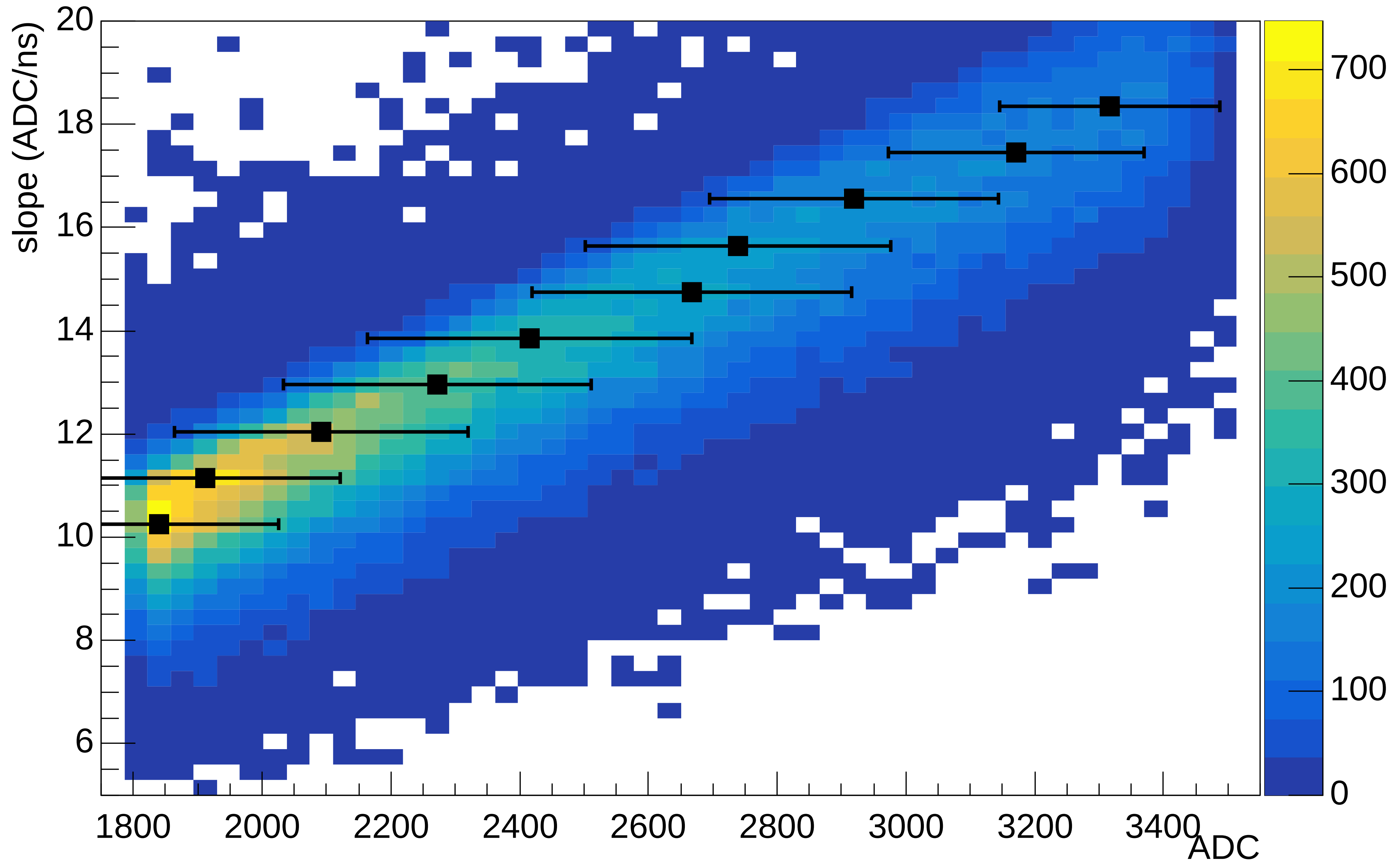
slope vs ADC
