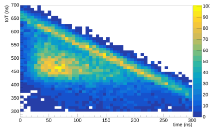
time vs TimeOverthreshold
