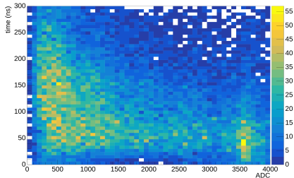
ADC vs time
