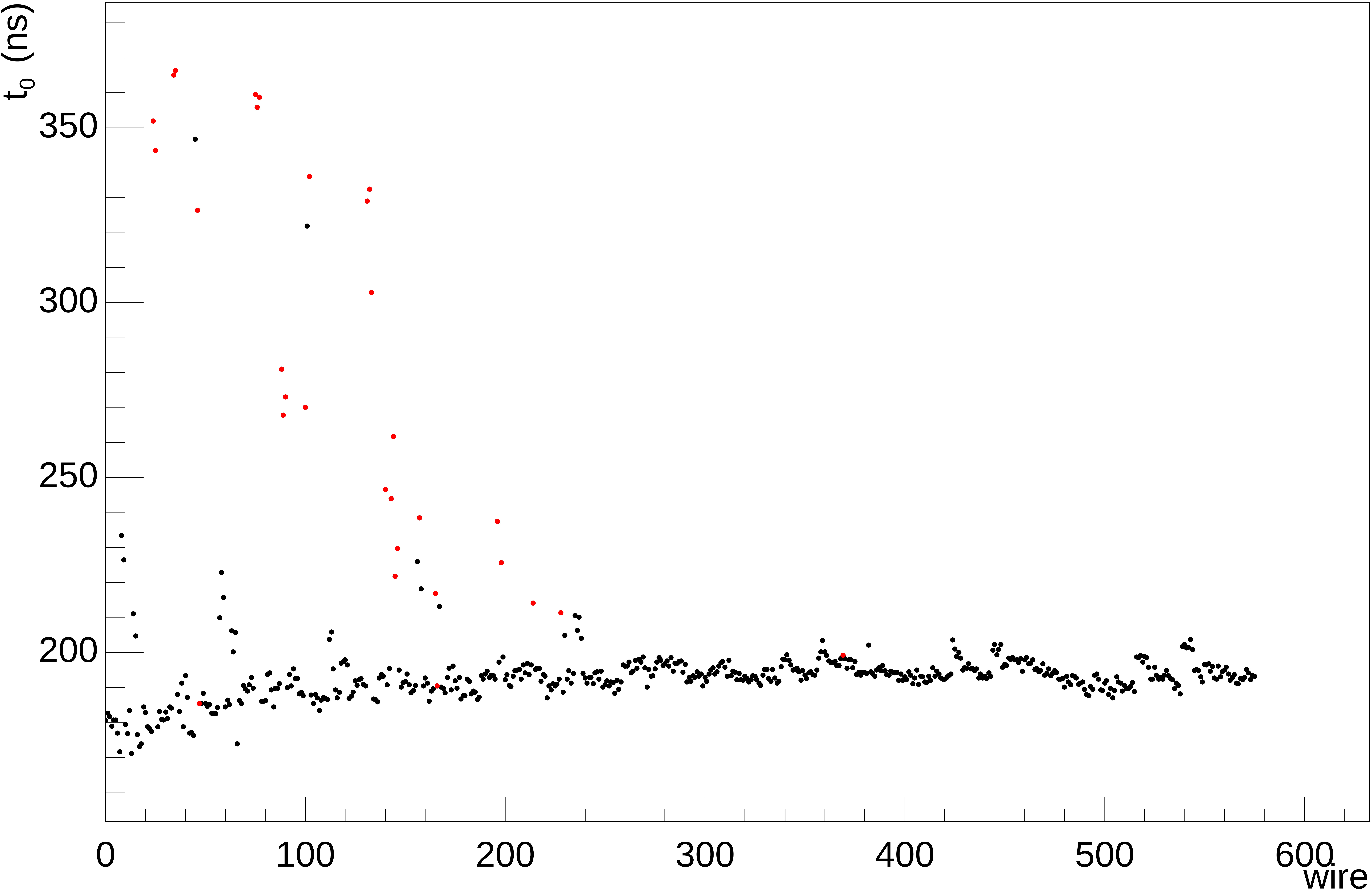
t_0 versus wire , run 22712, timestamp : May 04, 2026
