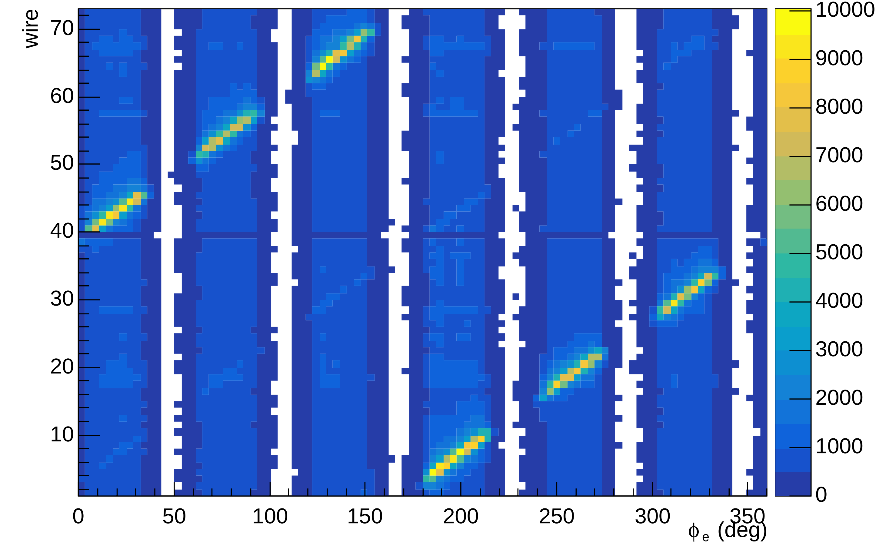
Wire occupation versus Electron phi (layer 32)
