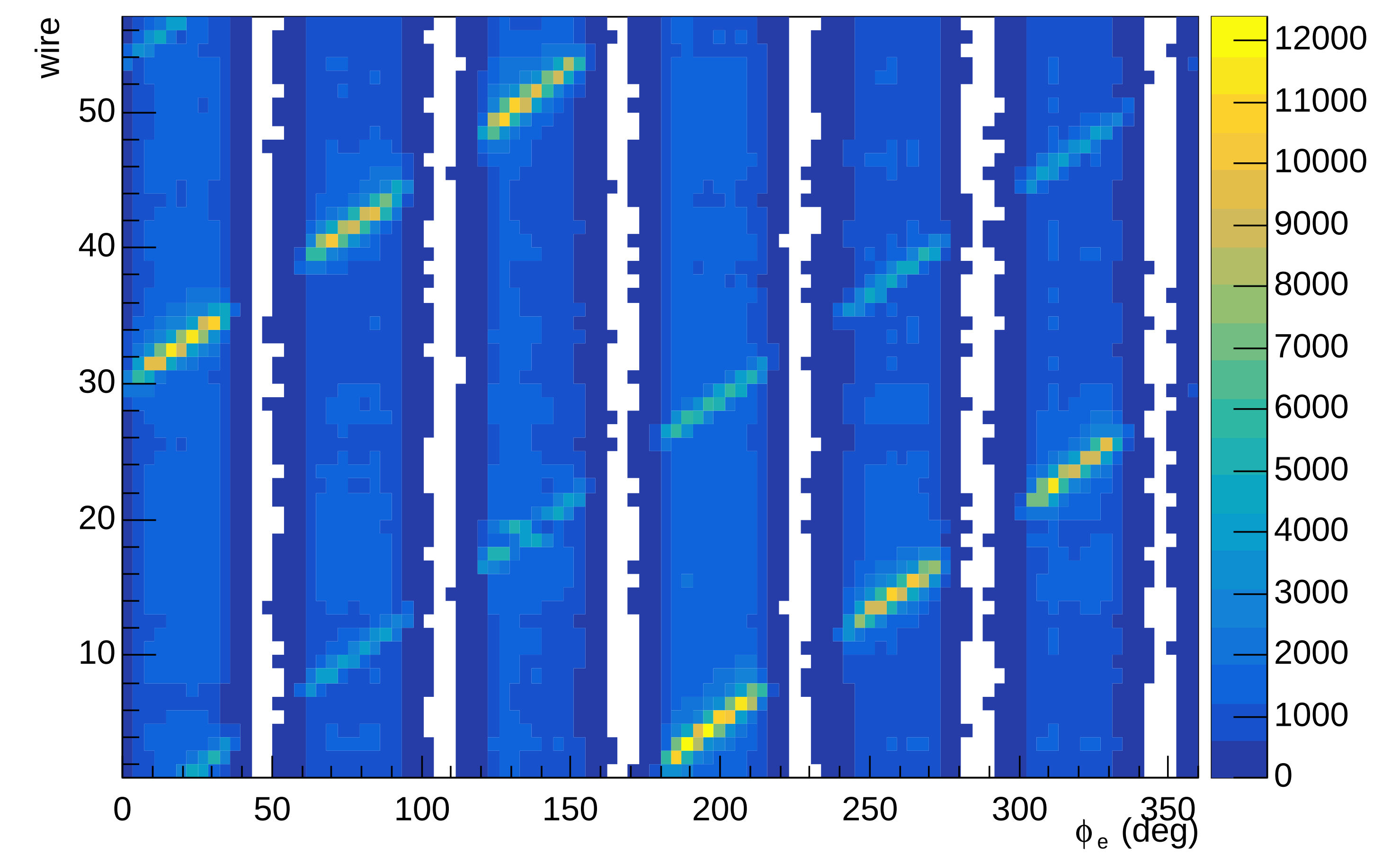
Wire occupation versus Electron phi (layer 21)
