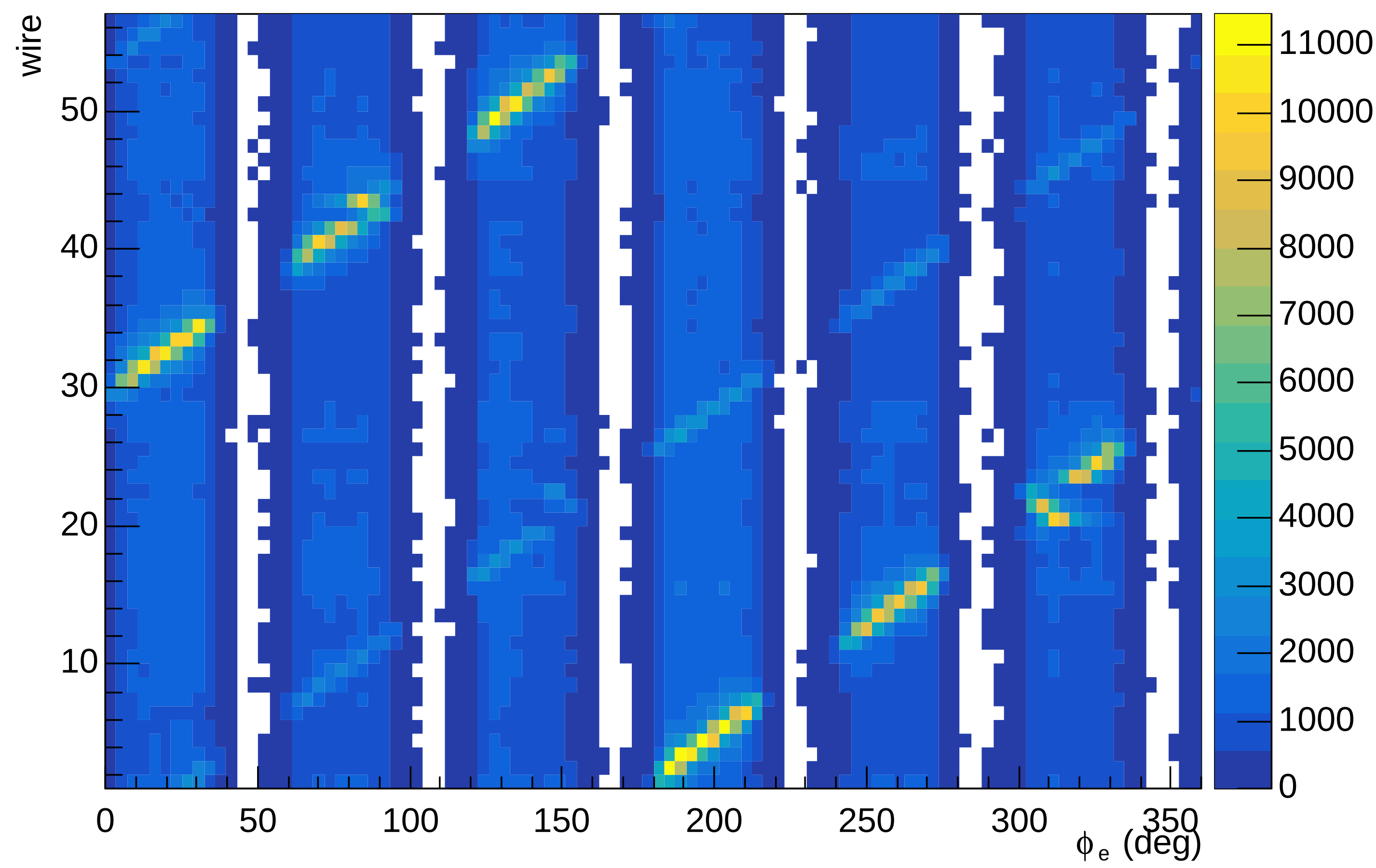
Wire occupation versus Electron phi (layer 22)
