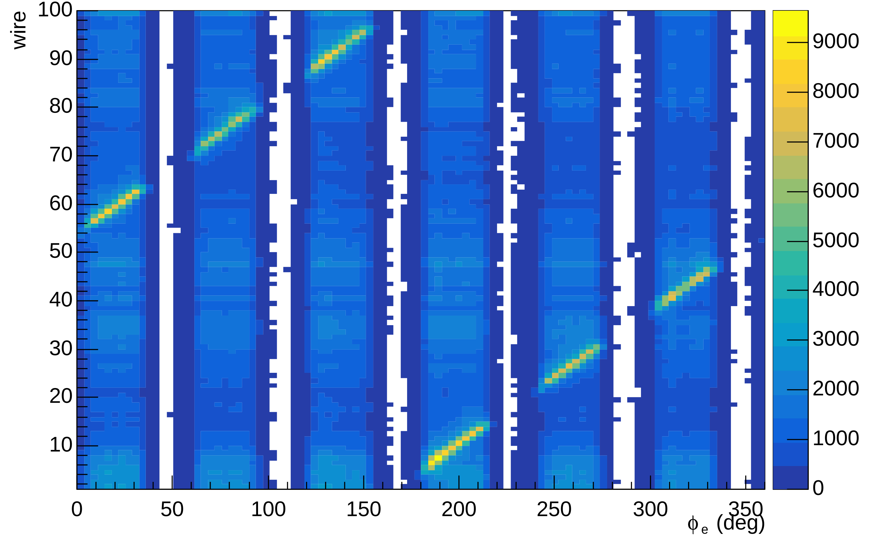
Wire occupation versus Electron phi (layer 51)
