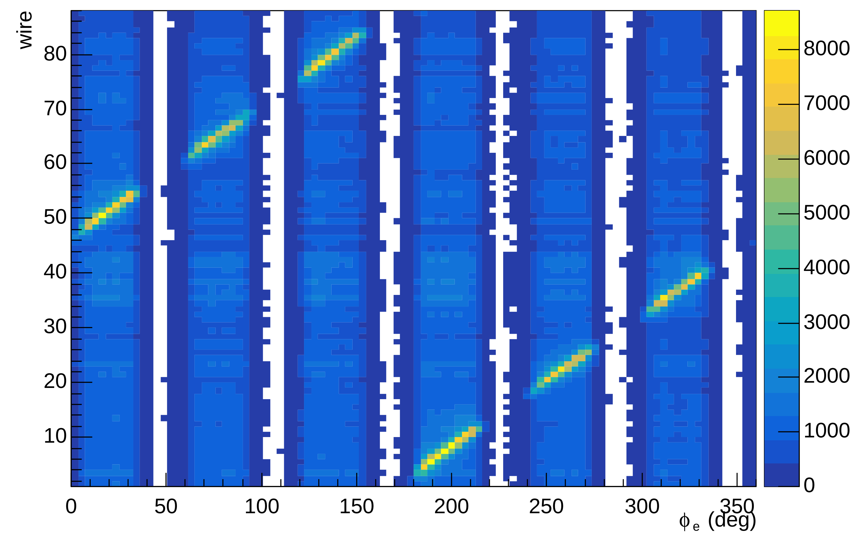
Wire occupation versus Electron phi (layer 42)
