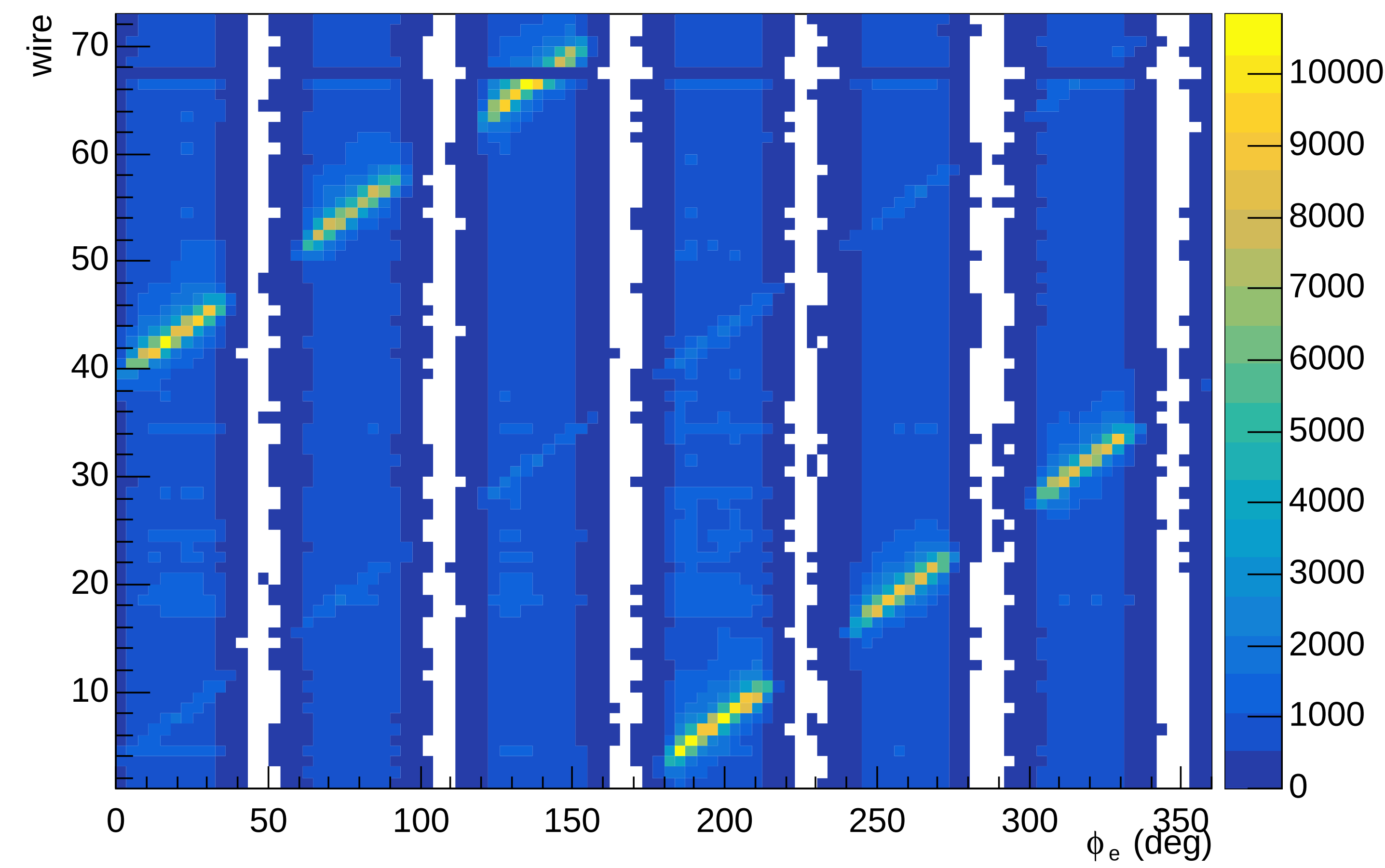
Wire occupation versus Electron phi (layer 31)
