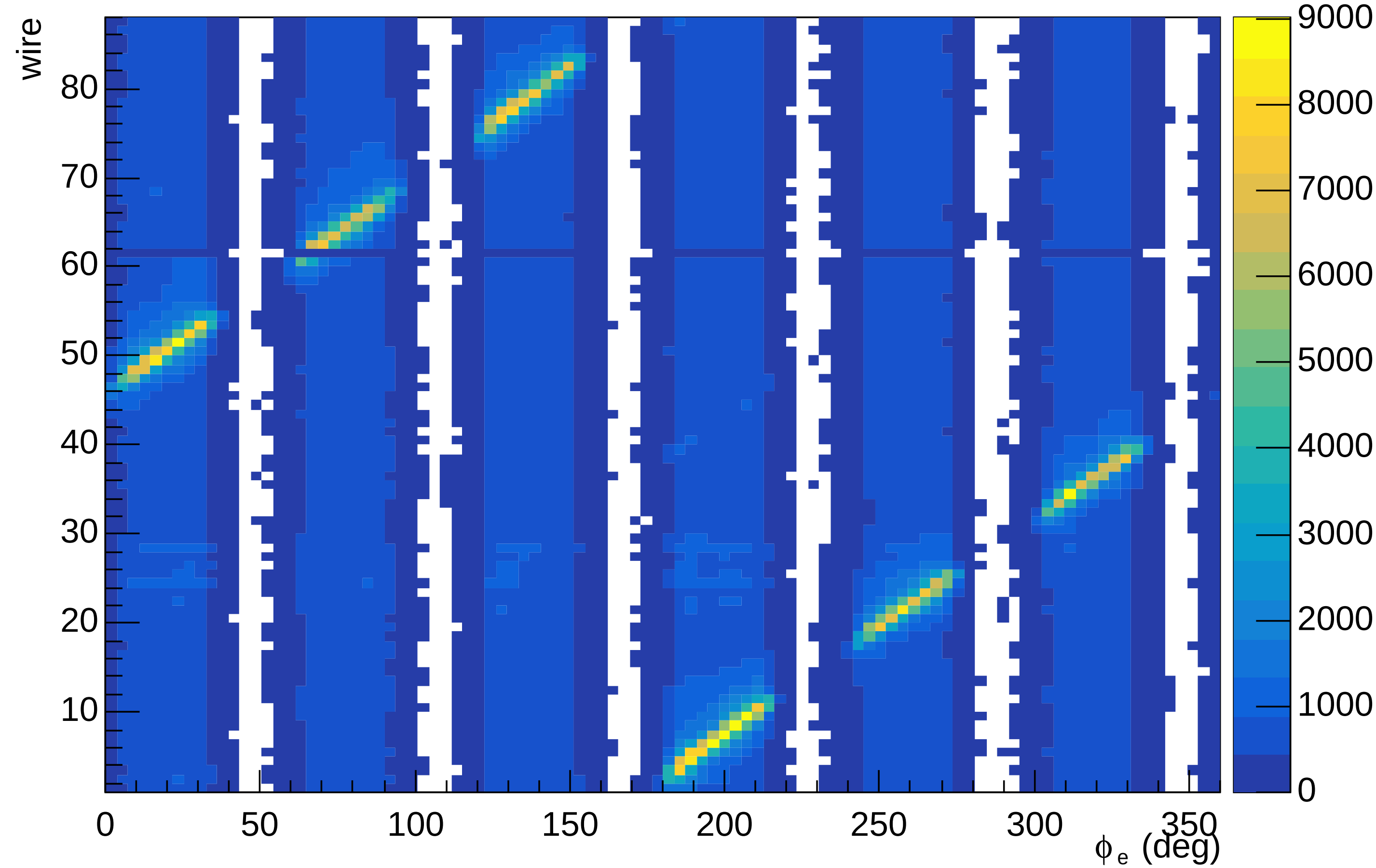
Wire occupation versus Electron phi (layer 41)
