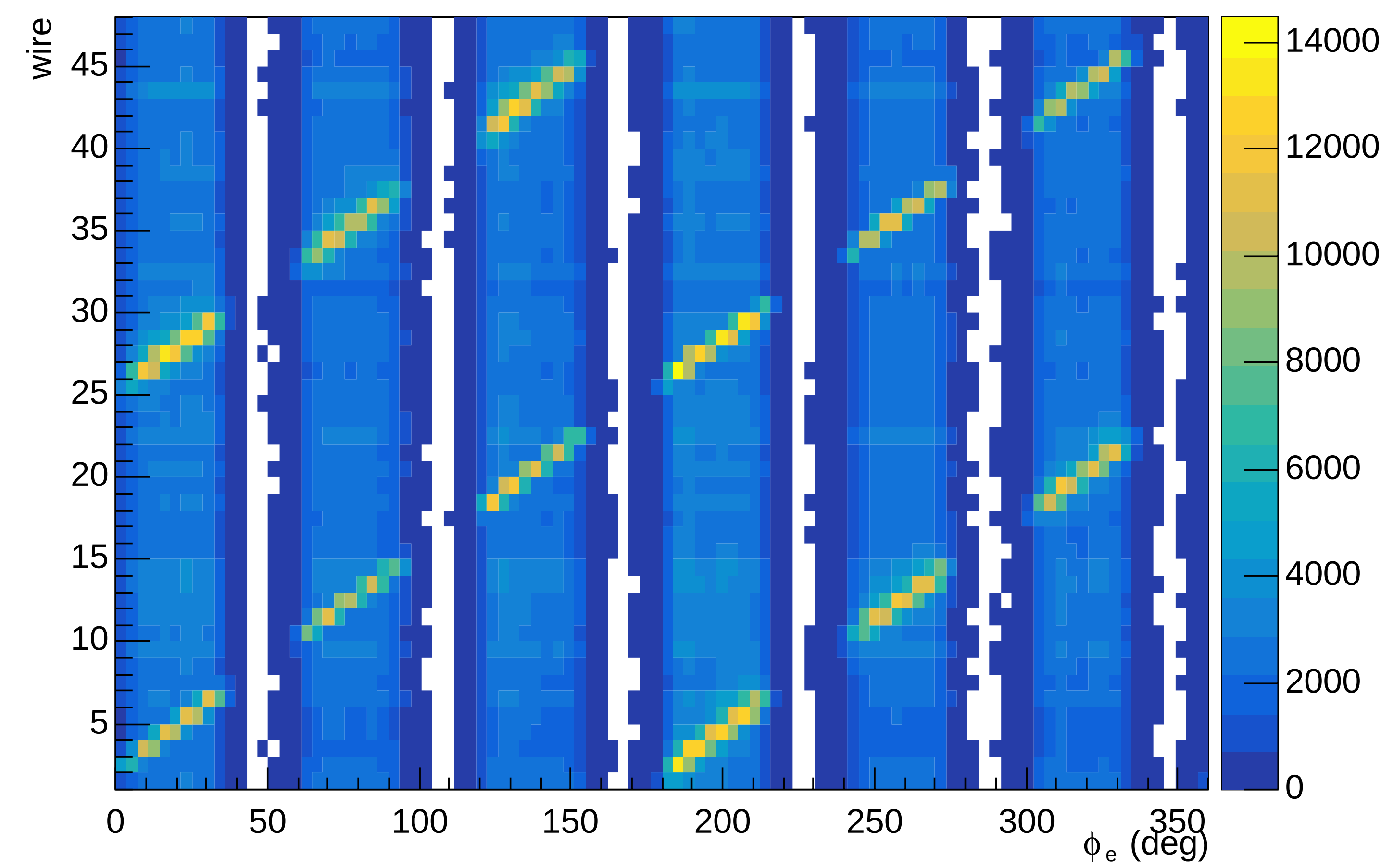
Wire occupation versus Electron phi (layer 11)
