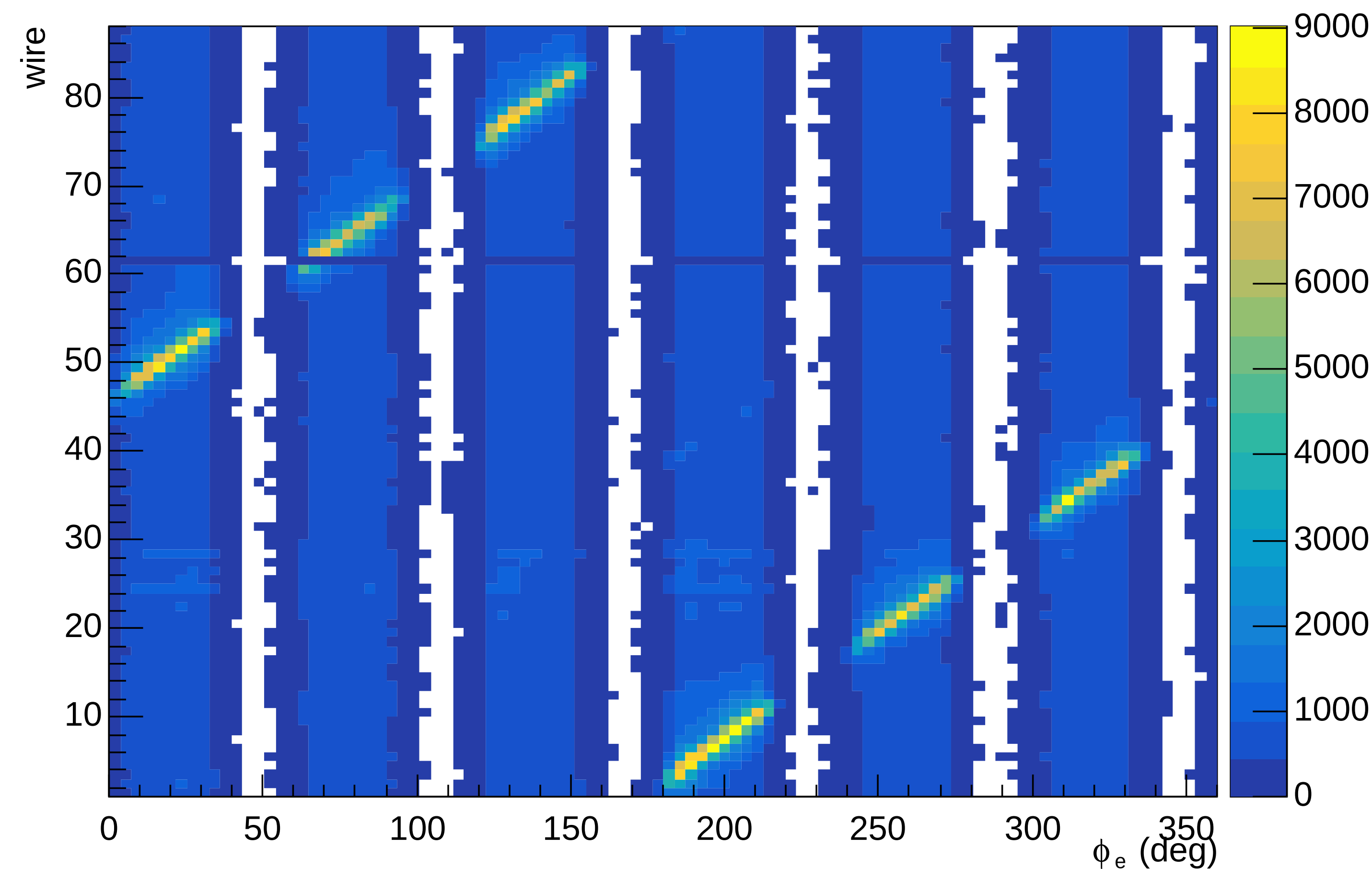
Wire occupation versus Electron phi (layer 41)
