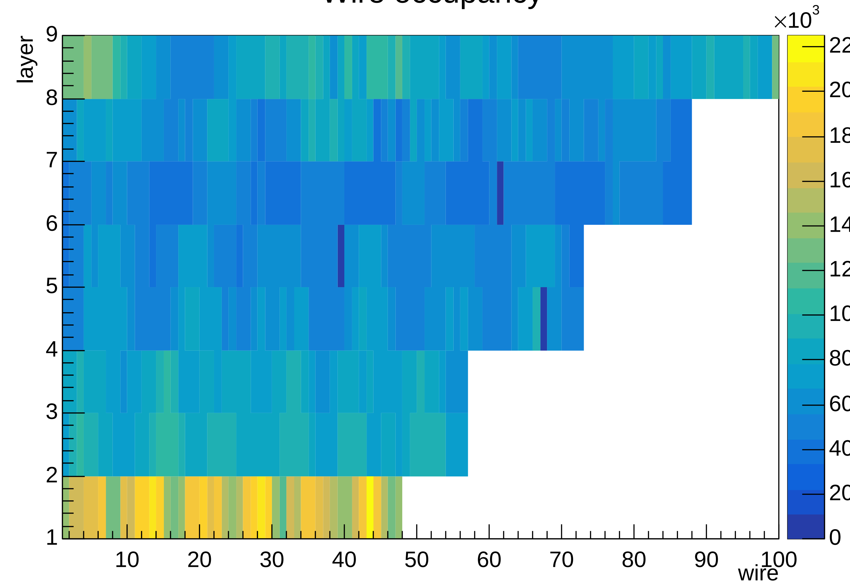
Wire occupancy
