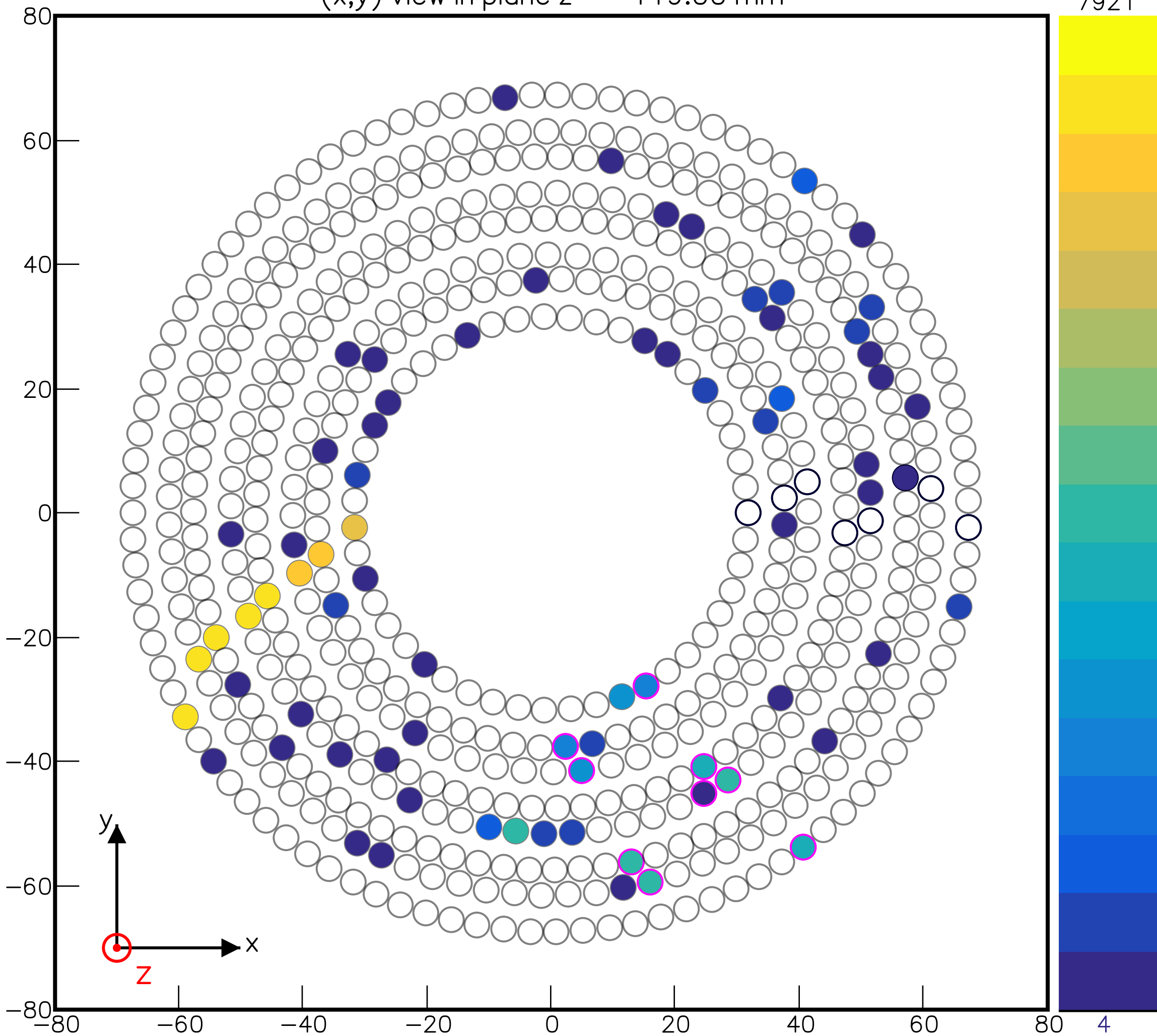
(x,y) view in plane z = -119.00 mm
