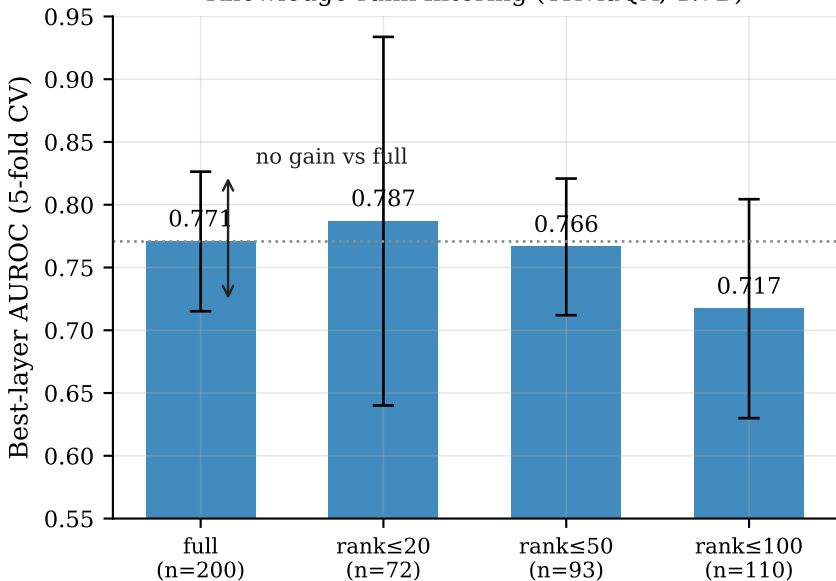
Knowledge-rank filtering (TriviaQA, 1.7B)
