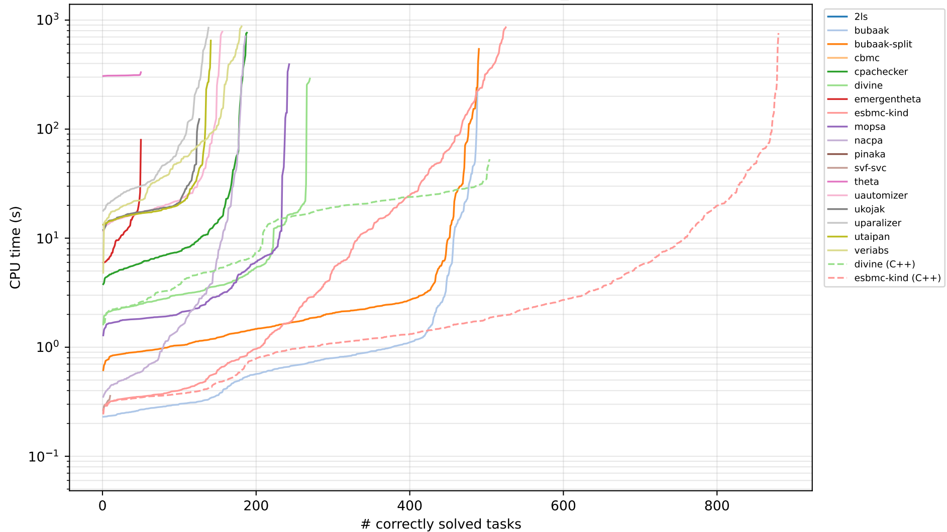
Quantile plot — shared cpp-baseline n c-exact_std (983 tasks)
