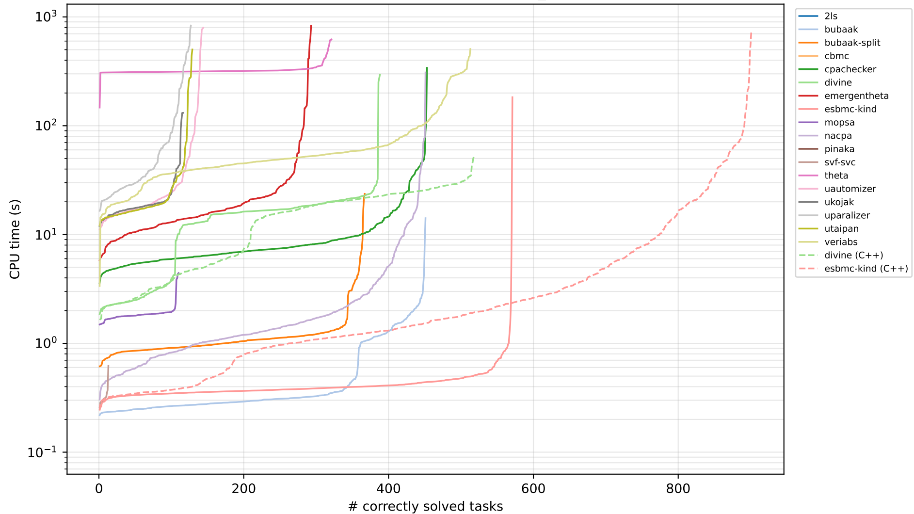
Quantile plot — shared cpp-baseline n c-havoc_std (1011 tasks)
