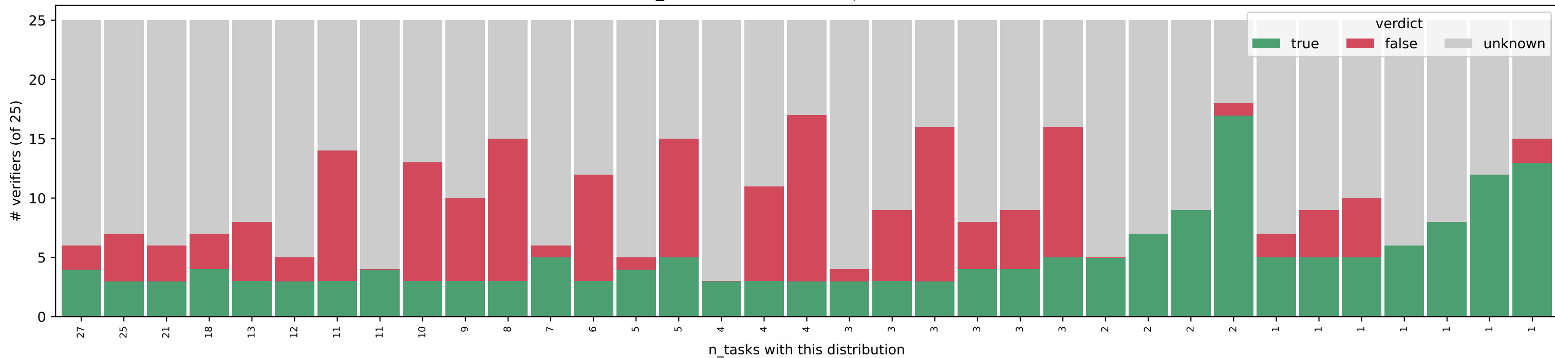
c-exact_std — label=true (62 patterns, 313 tasks)
