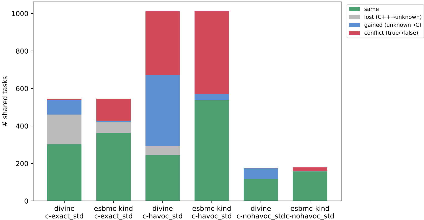
Per-tool verdict self-consistency: C++ original vs mapped-C
