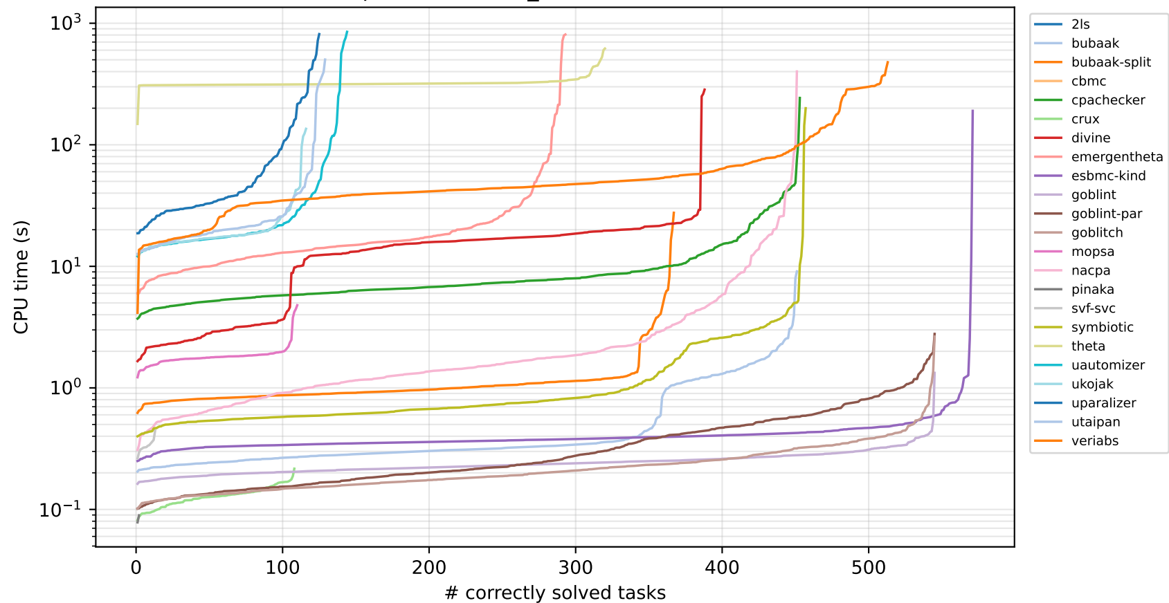
Quantile plot — c-havoc_std (23 verifiers solved \geq 1 )
