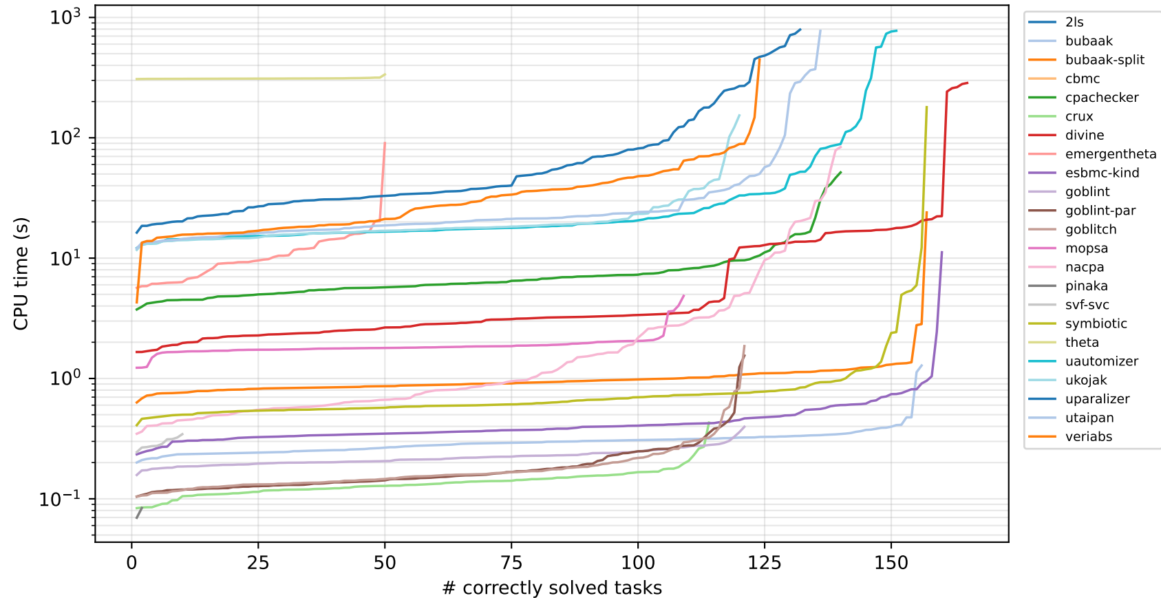
Quantile plot — c-nohavoc_std (23 verifiers solved \geq 1 )
