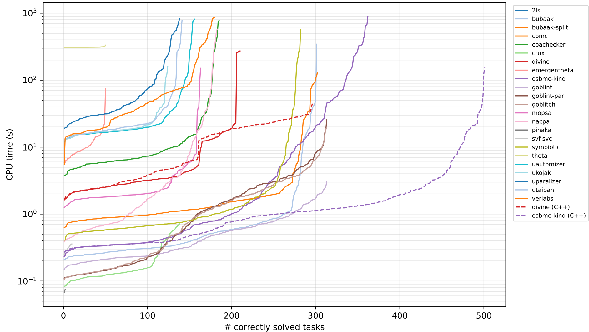
Quantile plot — shared cpp-baseline n c-exact_std (546 tasks)
