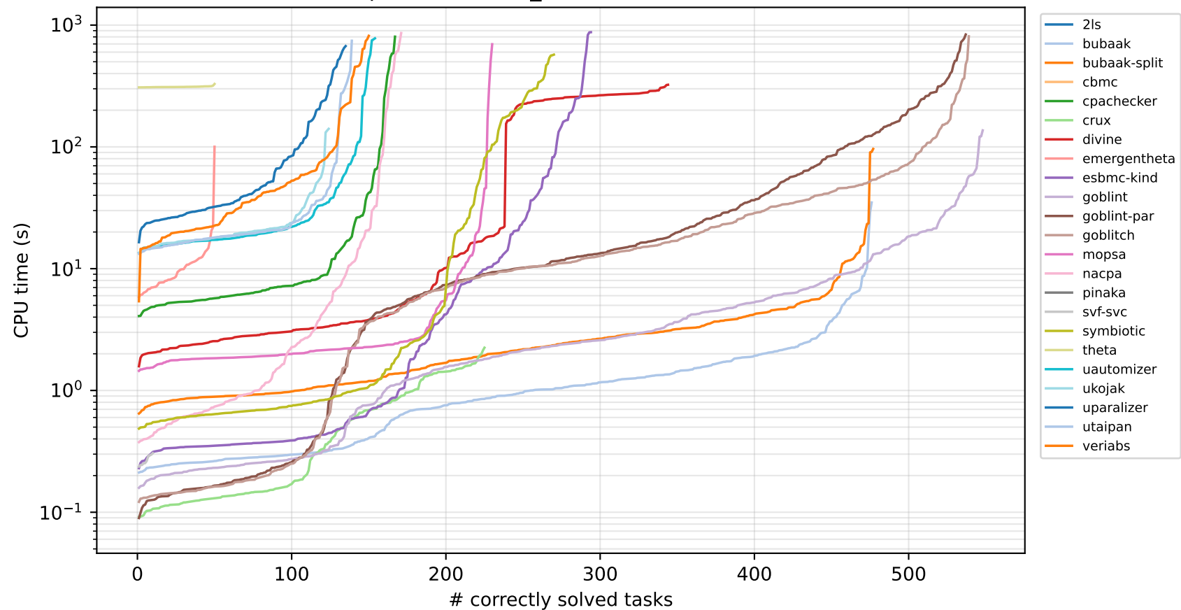
Quantile plot — c-exact_std (23 verifiers solved \geq 1 )
