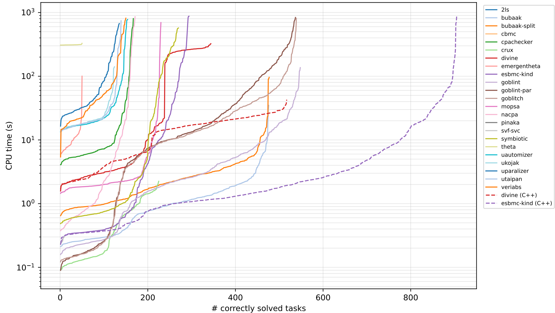
Quantile plot — shared cpp-baseline n c-exact std (1010 tasks)
