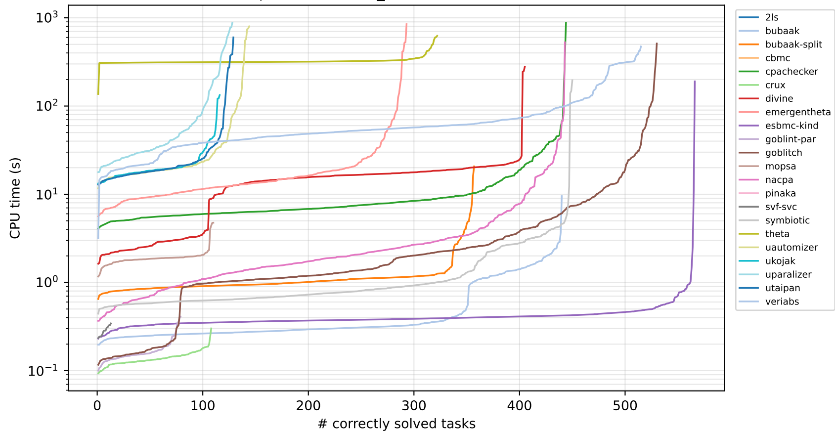
Quantile plot — c-havoc_std (22 verifiers solved \geq 1 )
