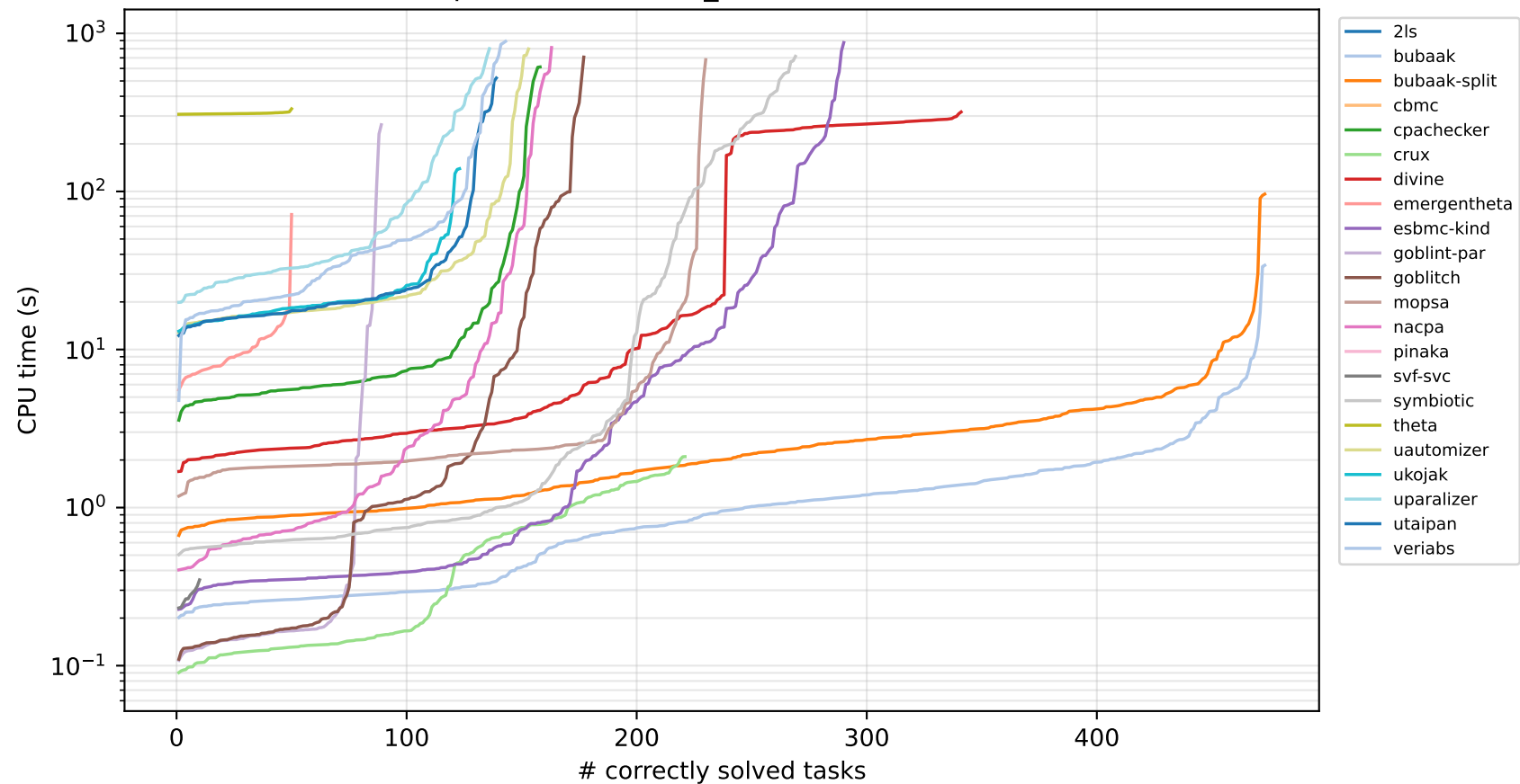
Quantile plot — c-nohavoc_std (22 verifiers solved \geq 1 )
