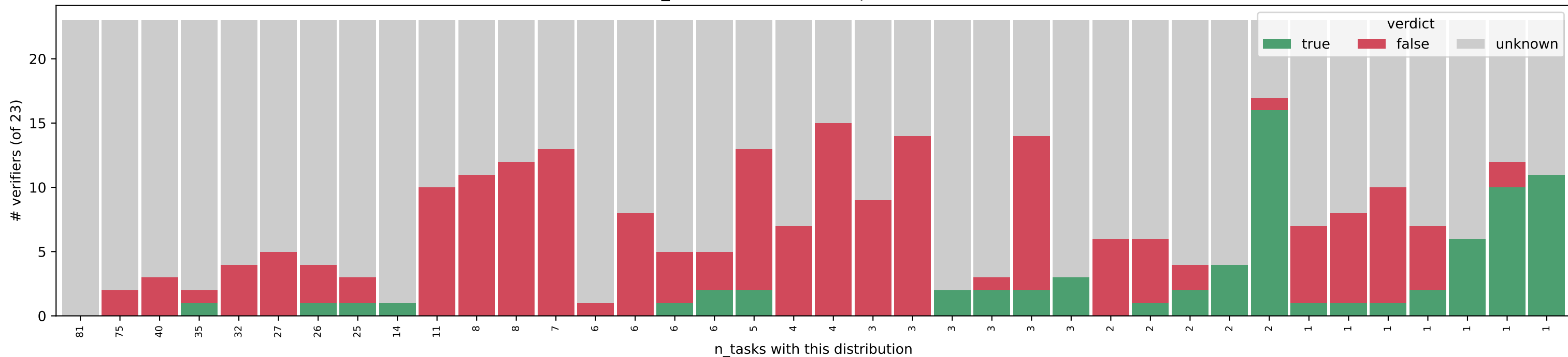
c-exact_std — label=true (61 patterns, 549 tasks)
