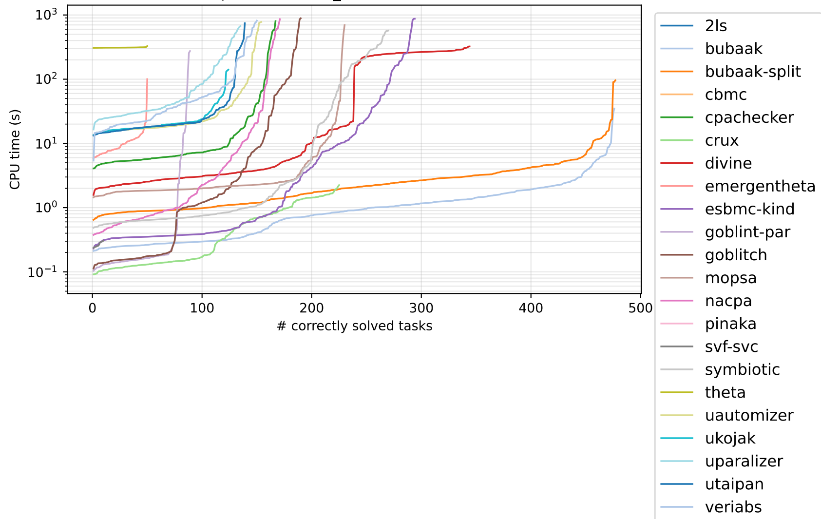
Quantile plot — c-exact_std (22 verifiers solved \geq 1 )
