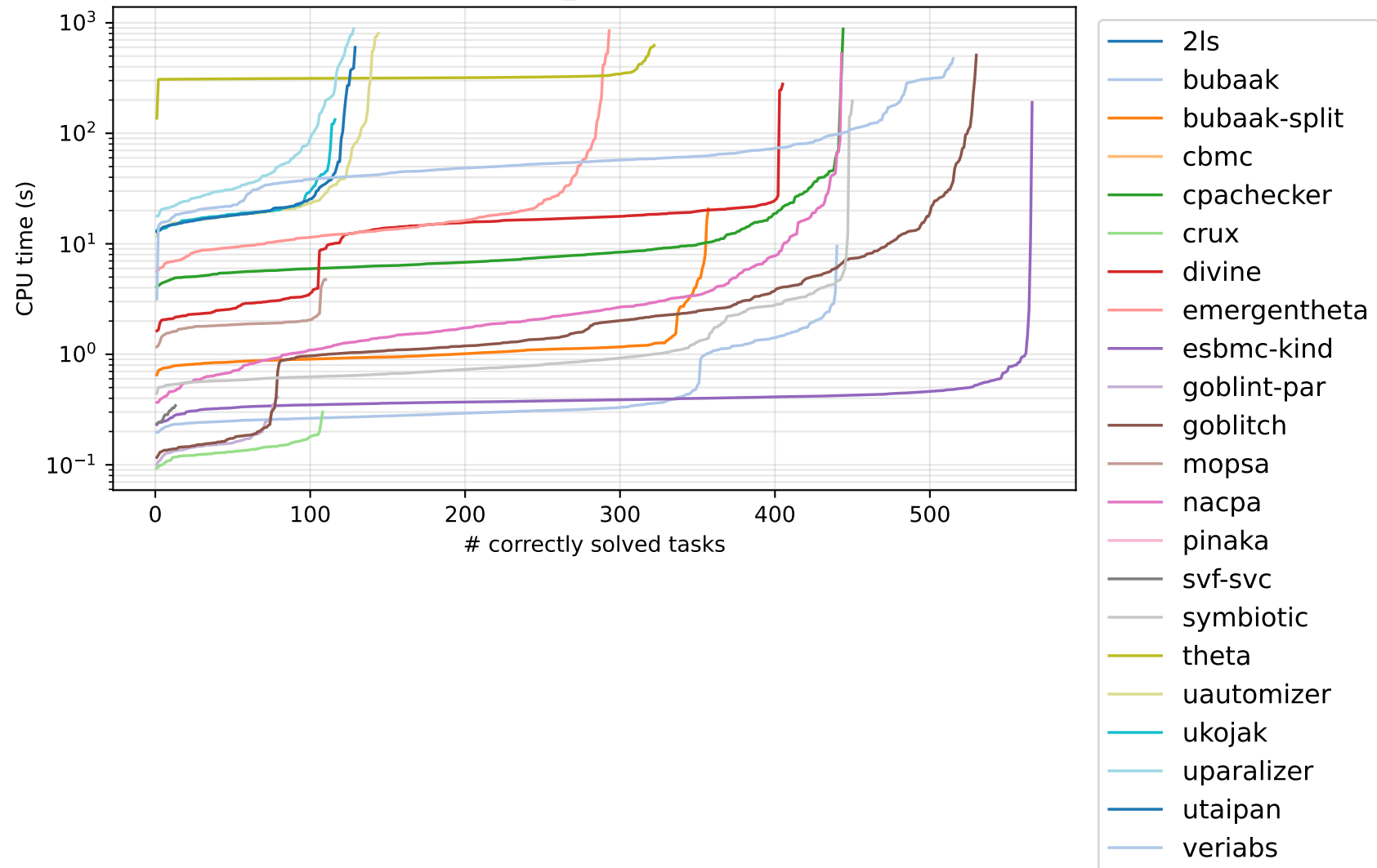
Quantile plot — c-havoc_std (22 verifiers solved \geq 1 )
