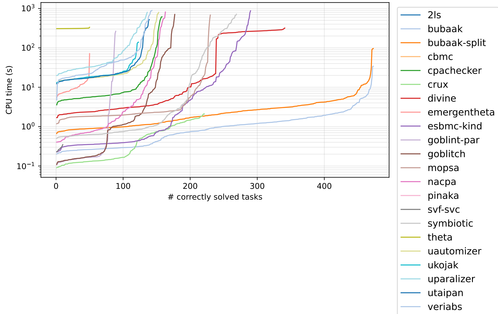
Quantile plot — c-nohavoc_std (22 verifiers solved \geq 1 )
