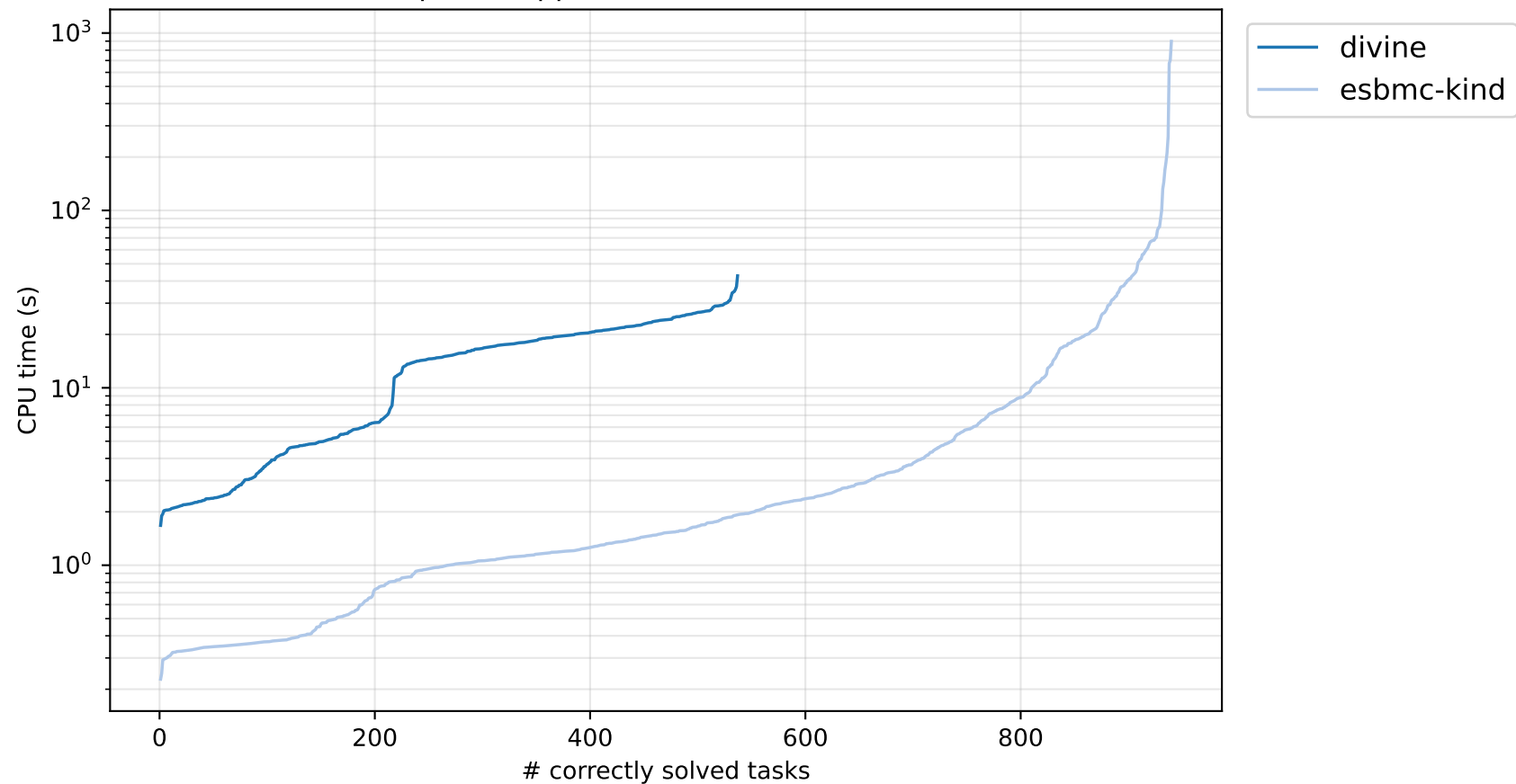
Quantile plot — cpp-baseline (2 verifiers solved \geq 1 )
