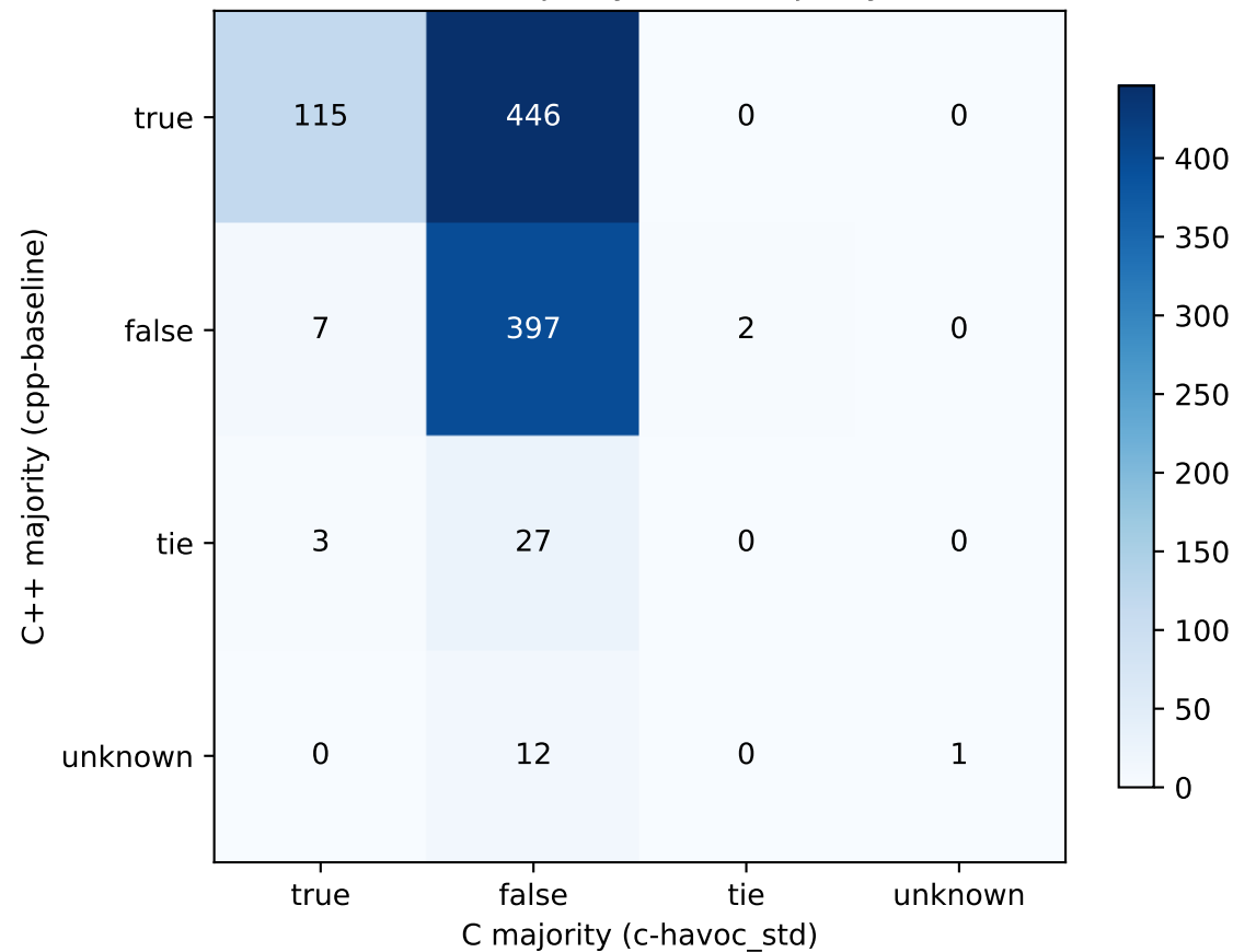
C++ majority vs. C majority
