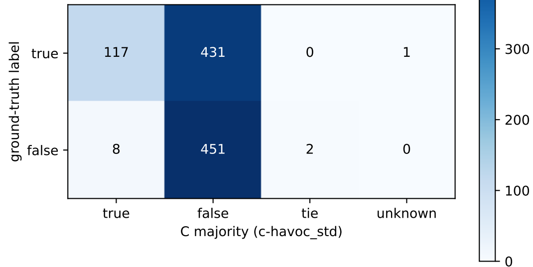
label vs. C majority
