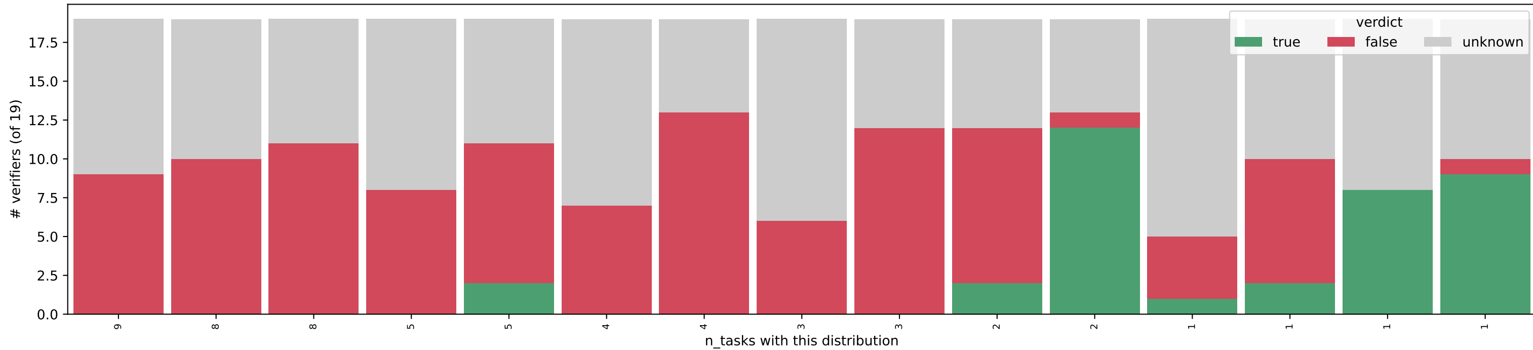
esbmc-eval-mapped-nostd — label=true (33 patterns, 121 tasks)
