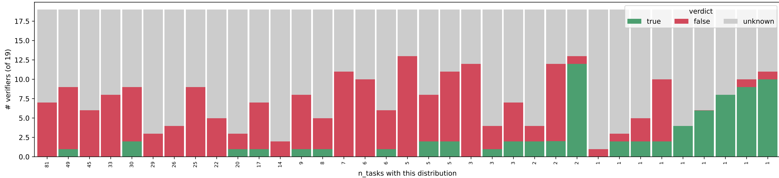
esbmc-eval-mapped — label=true (52 patterns, 545 tasks)
