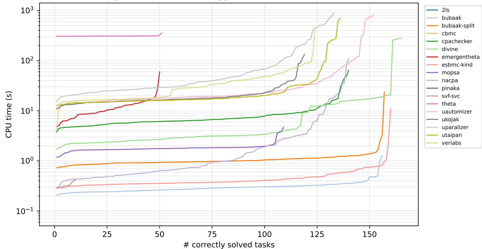
Quantile plot — esbmc-eval-mapped-nostd (18 verifiers solved \geq 1 )
