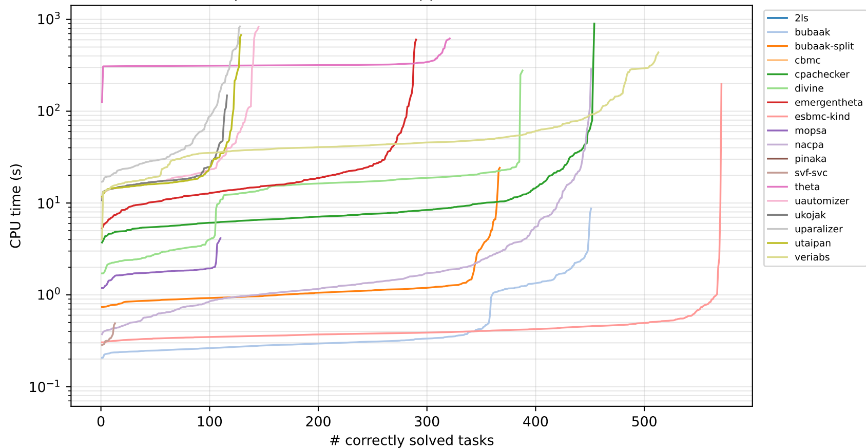
Quantile plot — esbmc-eval-mapped (18 verifiers solved \geq 1 )
