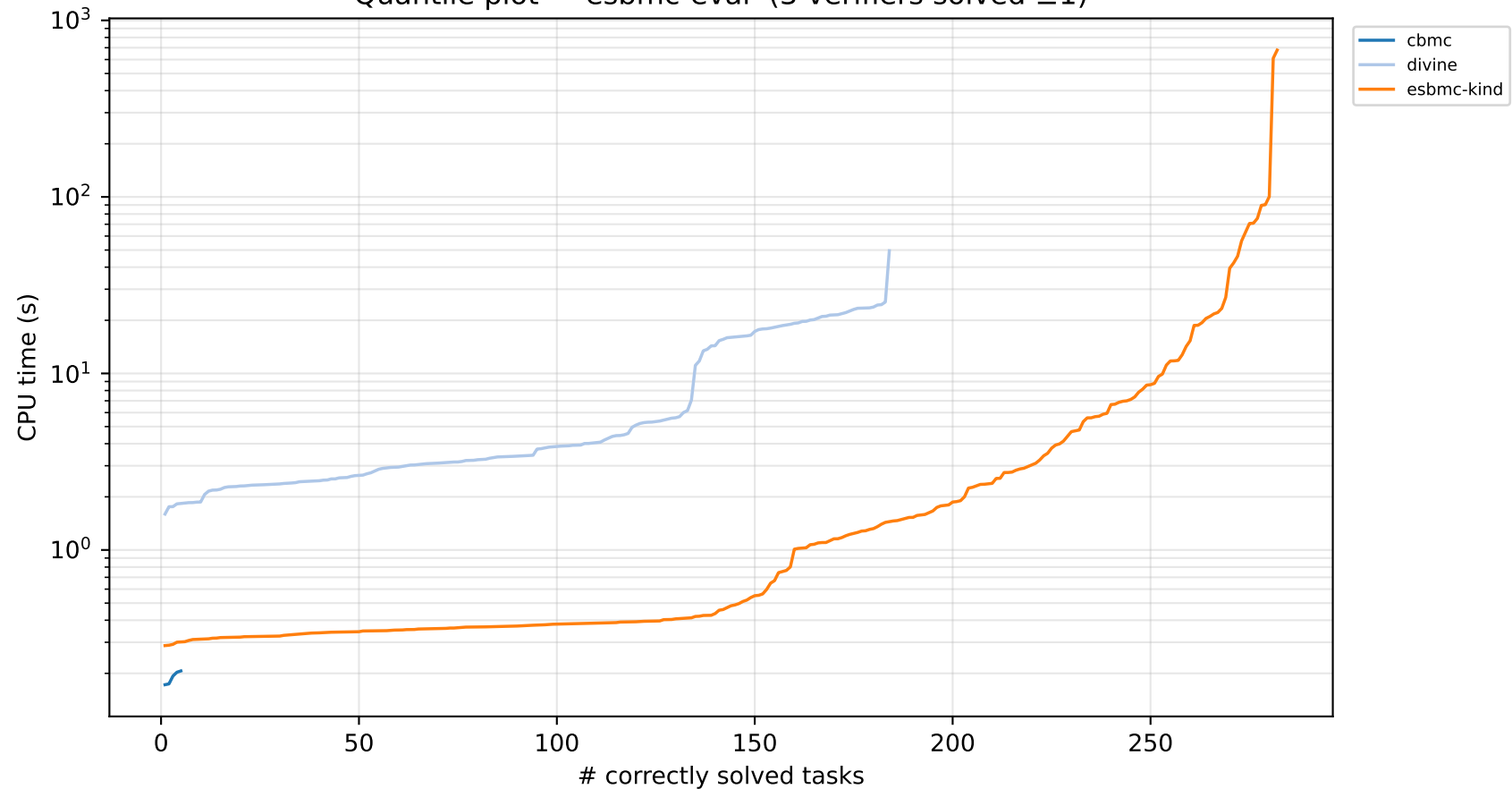
Quantile plot — esbmc-eval (3 verifiers solved \geq 1 )
