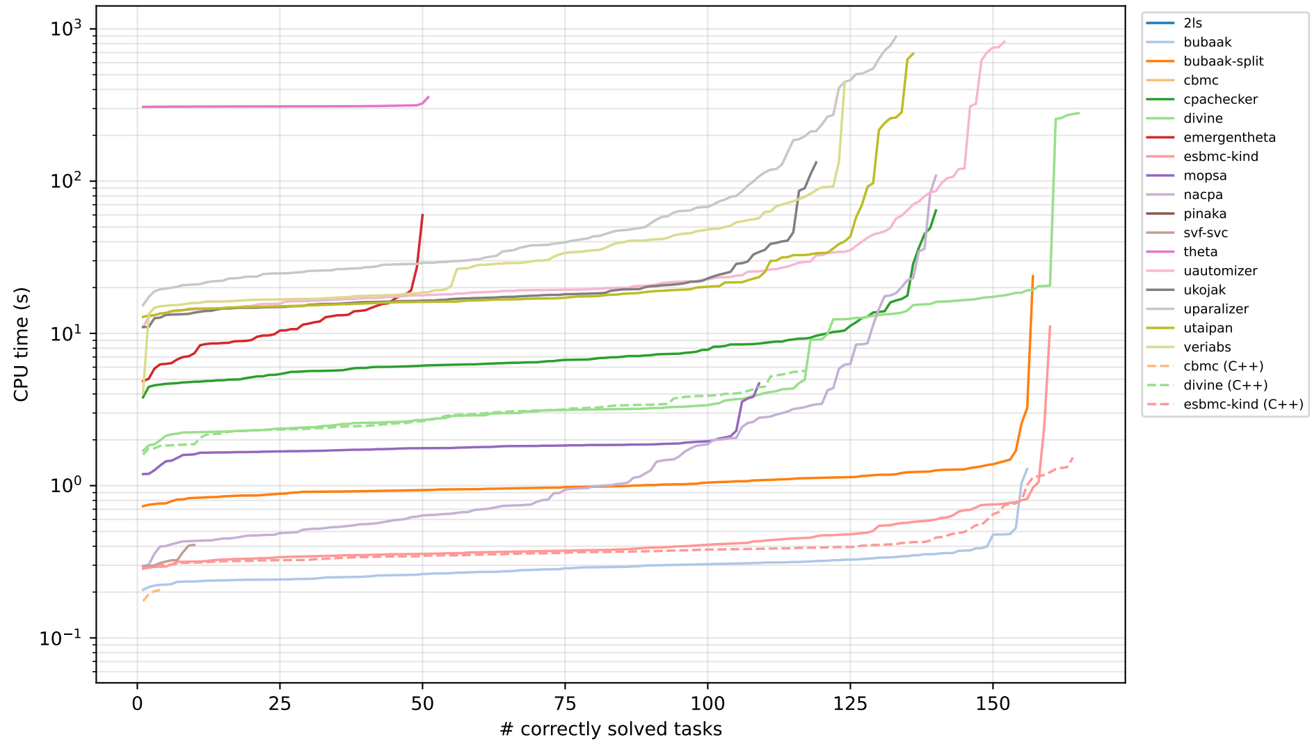
Quantile plot — shared esbmc-eval n esbmc-eval-mapped-nostd (178 tasks)
