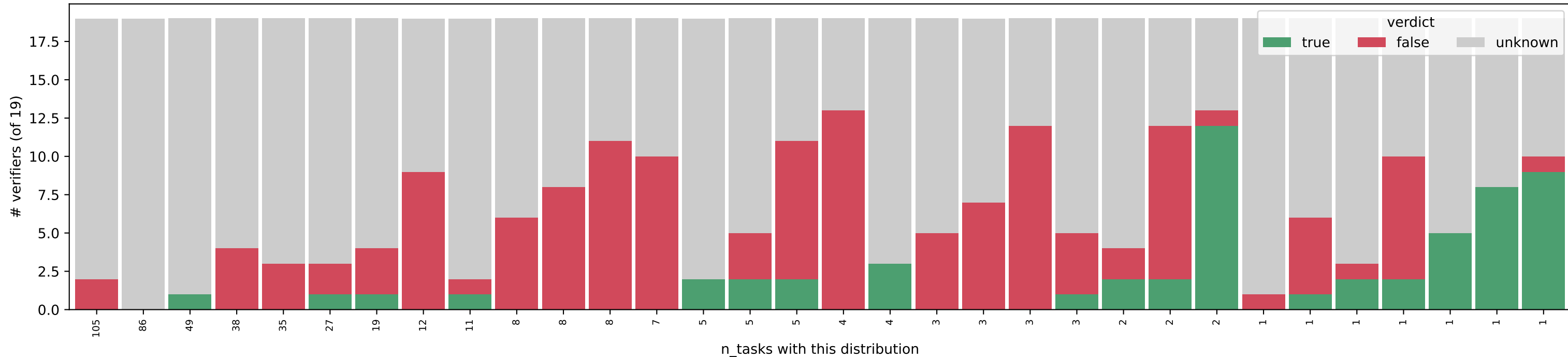
c-exact_std — label=true (48 patterns, 549 tasks)
