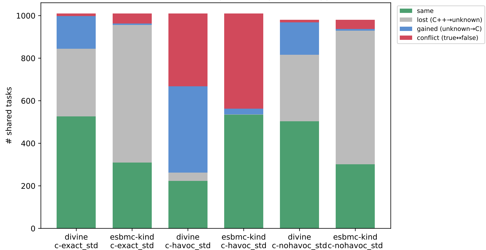
Per-tool verdict self-consistency: C++ original vs mapped-C
