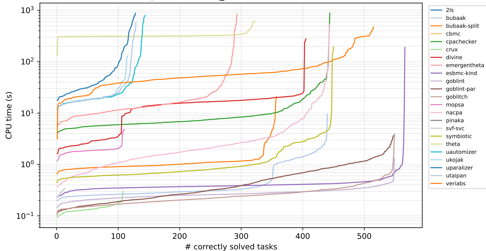
Quantile plot — c-havoc_std (23 verifiers solved \geq 1 )
