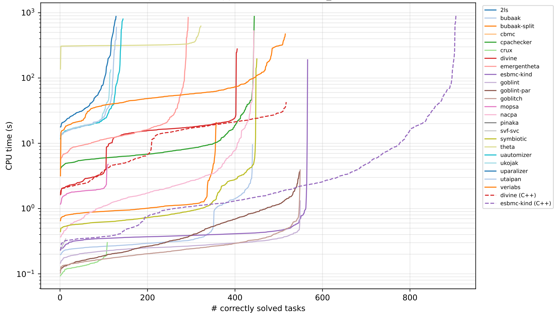
Quantile plot — shared cpp-baseline n c-havoc_std (1010 tasks)
