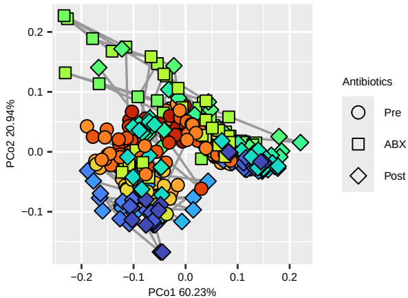
Weighted unifracs
