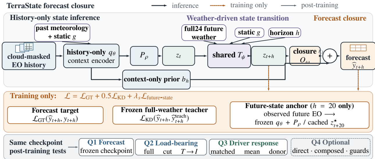
Figure 1: TerraState’s solid inference path is history-only: cloud-masked EO history, retained past meteorology, and static geography enter q_\theta , which emits the context-only prior b_h and, through P_\rho , the spatial state z_t . Full24 future weather, static geography, and horizon h condition the shared T_\psi ; the state contribution O_\omega(z_{t+h}) is then added explicitly to b_h . The orange band contains only training supervision: the ground-truth forecast loss, distillation from a frozen full-weather teacher, and the h = 20 future-state anchor from a frozen future-observation encoder/cache. Neither teacher nor observed future enters inference. The bottom strip summarizes same-checkpoint post-training evidence: Q1 forecast skill, Q2 closure and transition cuts, Q3 matched weather controls, and optional Q4 direct/composed queries under endpoint and non-collapse guards.
