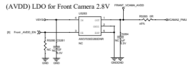
(AVDD) LDO for Front Camera 2.8V
